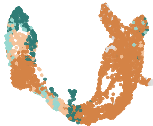
HarmoCycle
