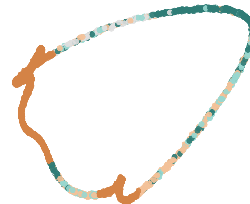
Spectral Topology
