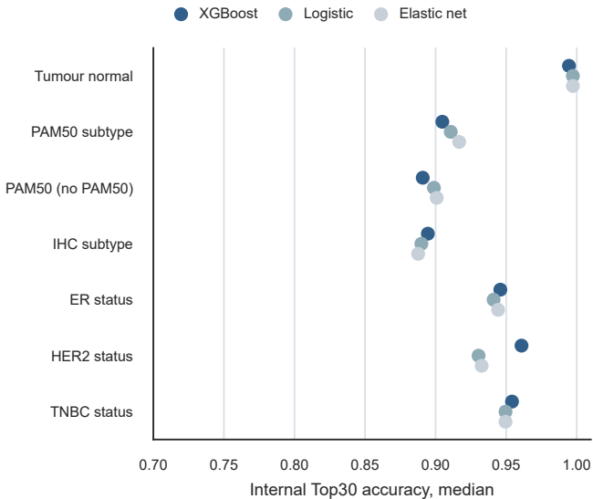
a Top30 baselines retain task signal
