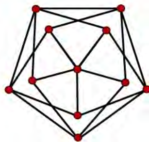
Figure 11.27 Graph G with no triangles and \chi(G) = 4 .
