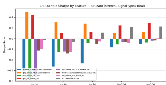
S&P 1500 (Stretch)
