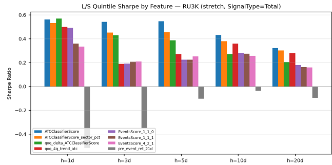
Russell 3000 (Stretch)
