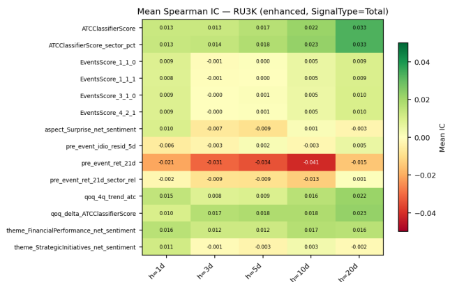
Russell 3000 (Enhanced)
