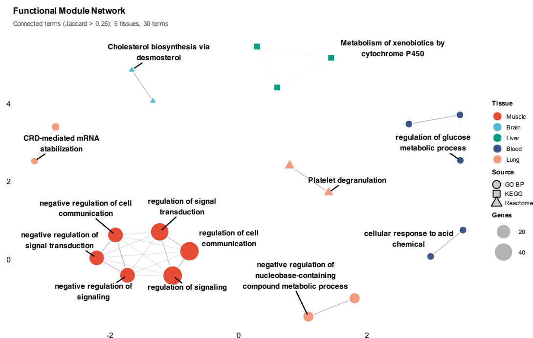
Figure 5.3: Functional enrichment analysis of stage-informative genes. Functional network showing interconnected enrichment modules, with nodes representing enriched terms coloured by tissue and edges connecting terms sharing >25% of genes (Jaccard similarity). Hubs and cluster representatives are labelled with biological process or pathway names.
