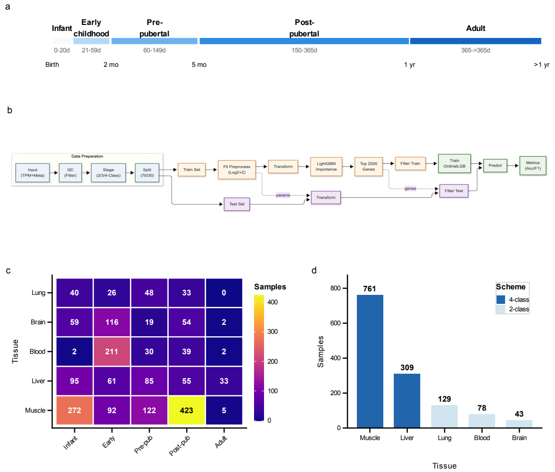
Figure 5.1: Study design and data landscape. (a) Developmental stage definitions mapping chronological age to five ordered stages: Infant (0–20 days), Early childhood (21–59 days), Pre-pubertal (60–149 days), Post-pubertal (150–365 days), and Adult (>365 days). (b) Machine learning workflow diagram illustrating the pipeline from data preprocessing to model calibration and evaluation. (c) Sample distribution heatmap showing tissue-by-stage availability across 1,924 samples from five tissues. (d) Classification scheme assignments based on per-class sample availability.
