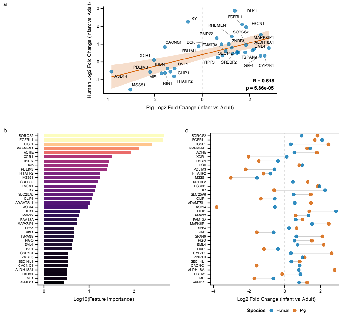
Figure 5.4: Cross-species validation of developmental gene expression. Human skeletal muscle transcriptomic data comparing infant (7–28 months) versus adult (30–56 years) samples were used to validate conservation of developmental signatures. (a) Scatter plot of log 2 fold changes between pig and human, showing significant positive correlation. (b) Feature importance of top conserved markers in the developmental stage classifier. (c) Paired fold change comparison showing pig and human values for each conserved gene.
