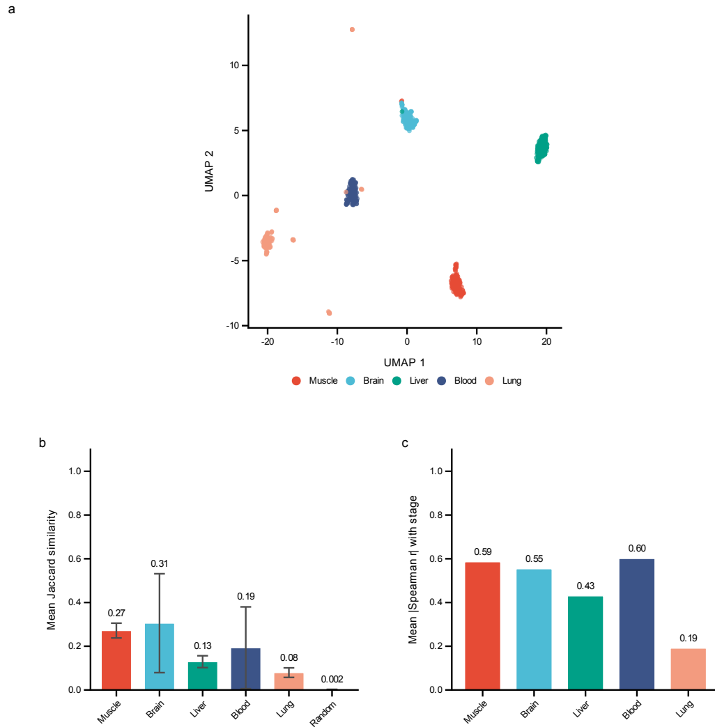
Figure S2: Tissue specificity and feature selection stability analysis. a , Uniform manifold approximation and projection (UMAP) (McInnes et al., 2020) of gene expression profiles across five tissues (muscle, brain, liver, blood, lung), demonstrating distinct tissue-specific clustering patterns ( n = 150 samples per tissue, balanced sampling; top 500 variable genes). For visualisation only, BioProject batch effects were removed per tissue using limma::removeBatchEffect (Ritchie et al., 2015) prior to UMAP; the machine learning pipeline operates on uncorrected expression data. b , Within-tissue feature selection stability quantified as mean Jaccard similarity index (Jaccard, 1912) of the top 50 selected features across ten independent random seeds. Error bars represent standard deviation; higher values indicate more reproducible feature selection. c , Mean absolute Spearman correlation between top-ranked features and developmental stage for each tissue.
