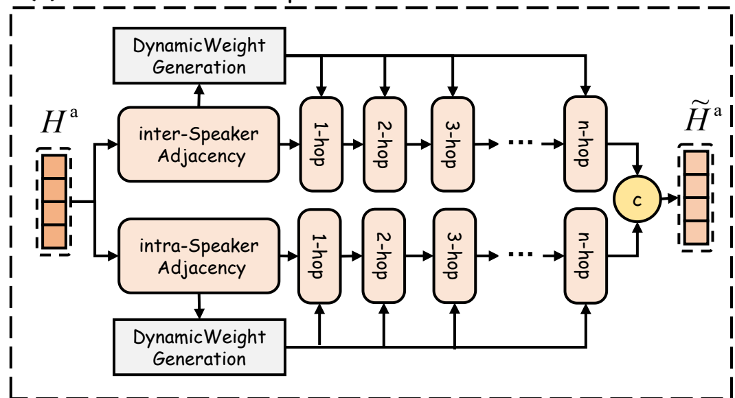
(b) Dual-Path Dynamic Multi-Hop Propagation
