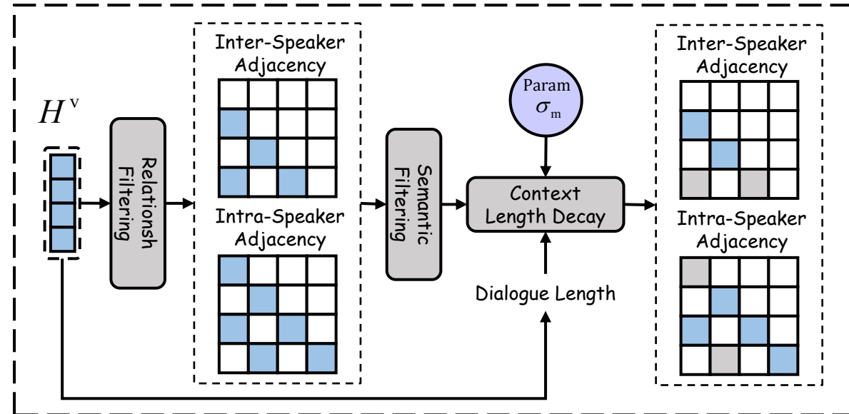
(a) Adaptive Neighbor Selection
