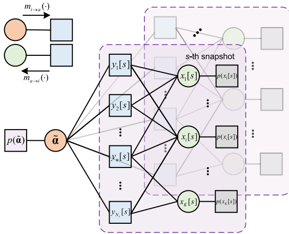
Fig. 10. The factor graph representation of the uplink ISAC receiver.
