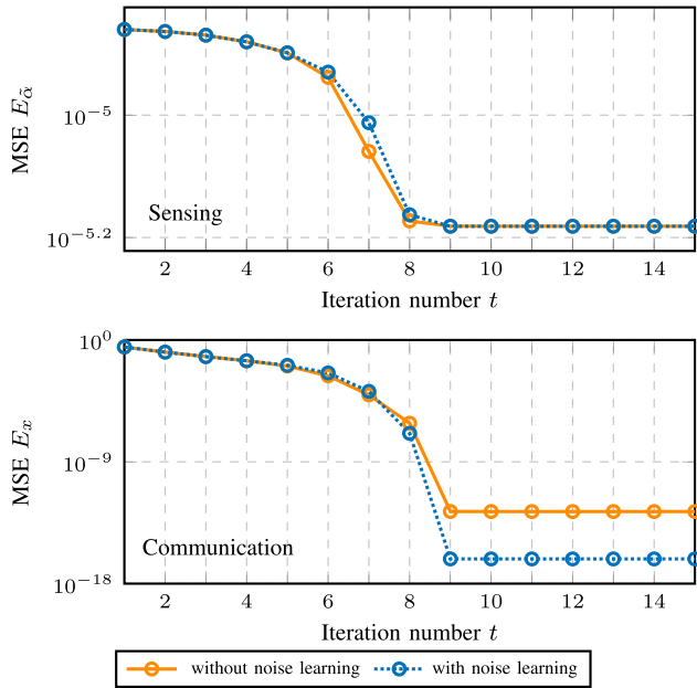
Fig. 3. MSEs performance of sensing and communication under 64-QAM with N_r = 40 , K = 20 , and L = 8 .
