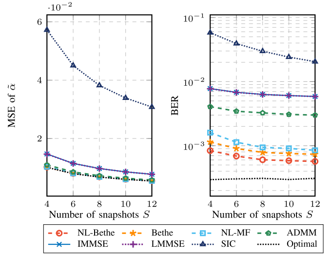
Fig. 8. MSE and BER performance of various methods with respect to the number of snapshots S .
