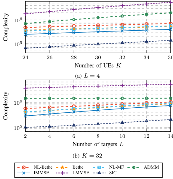
Fig. 9. Complexity comparisons of various methods with respect to (a) the number of UEs K and (b) the number of targets L .
