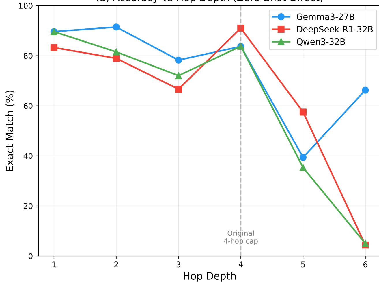
(a) Accuracy vs Hop Depth (Zero-Shot Direct)
