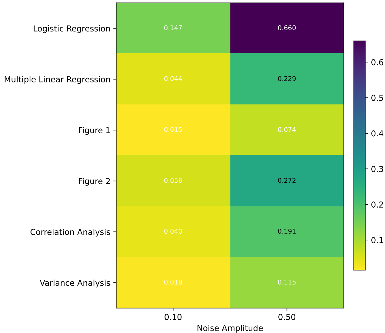
Mean Relative Result Error
