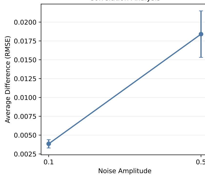
Correlation Analysis
