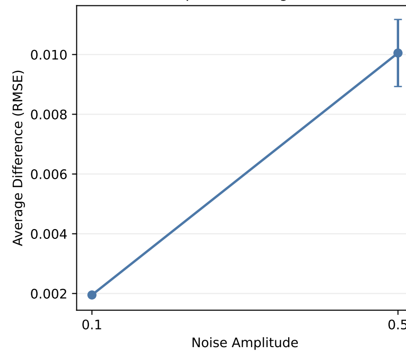
Correlation Analysis
