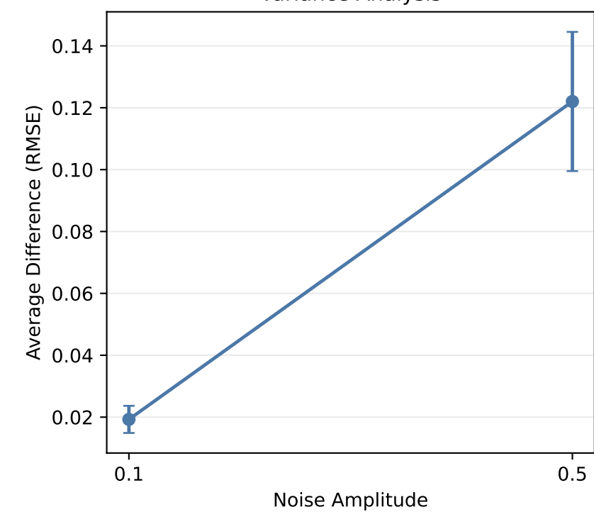
Variance Analysis
