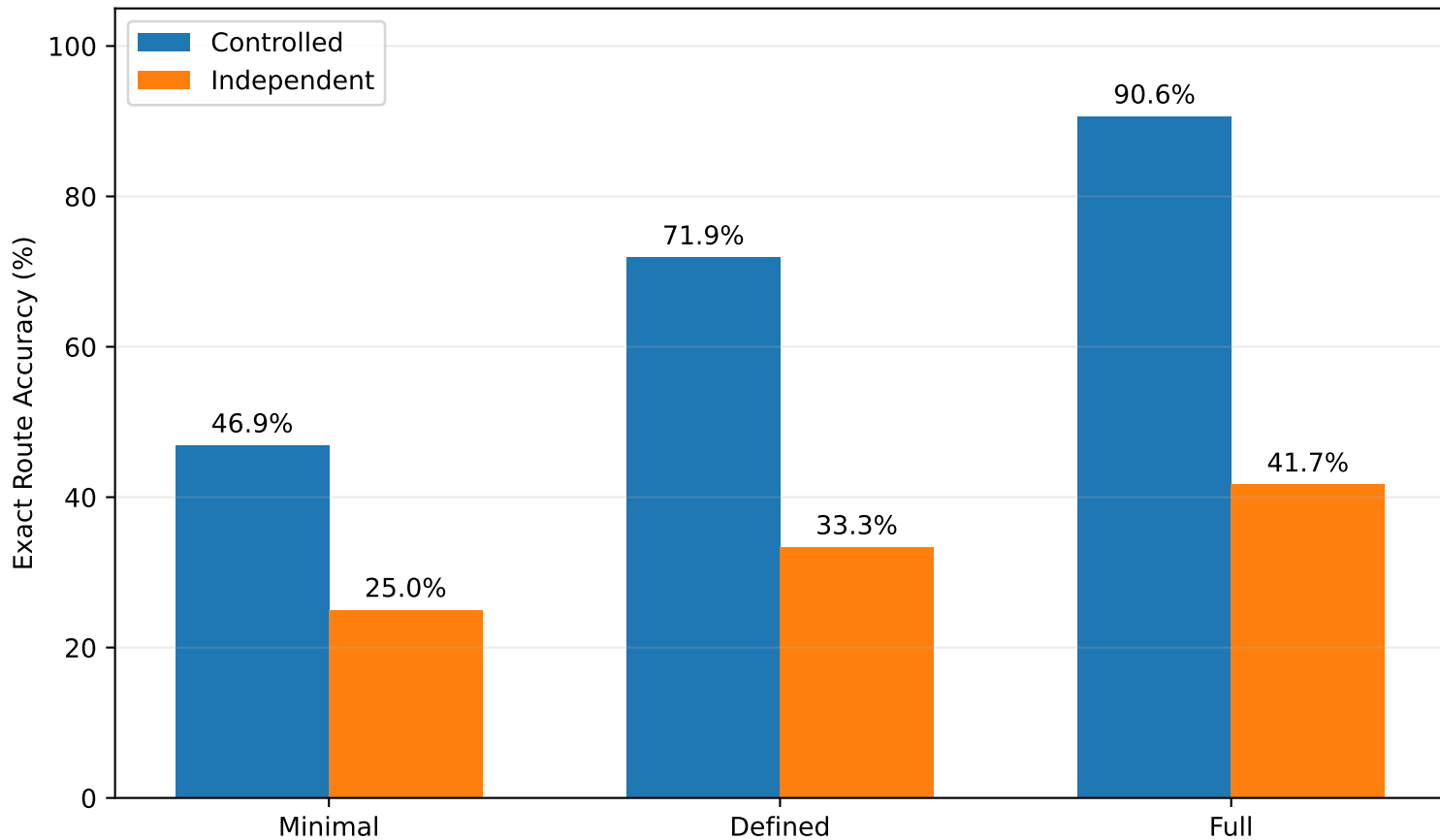
Privacy Prompt Design Ablation
