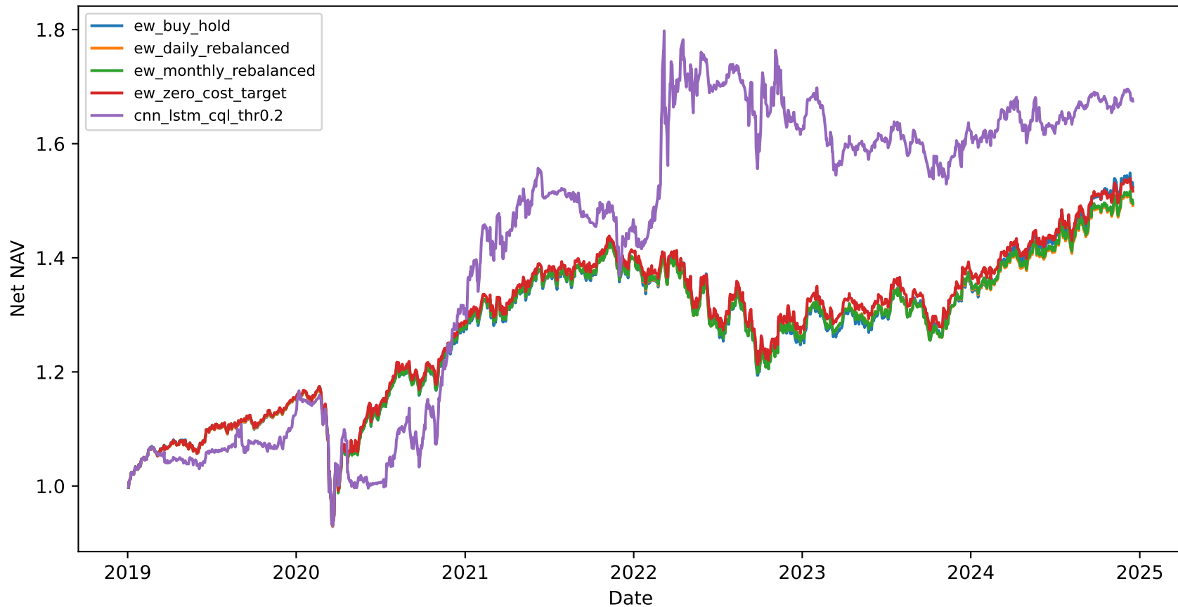
Full OOS NAV: fair equal-weight variants vs CNN-LSTM CQL-FQI
