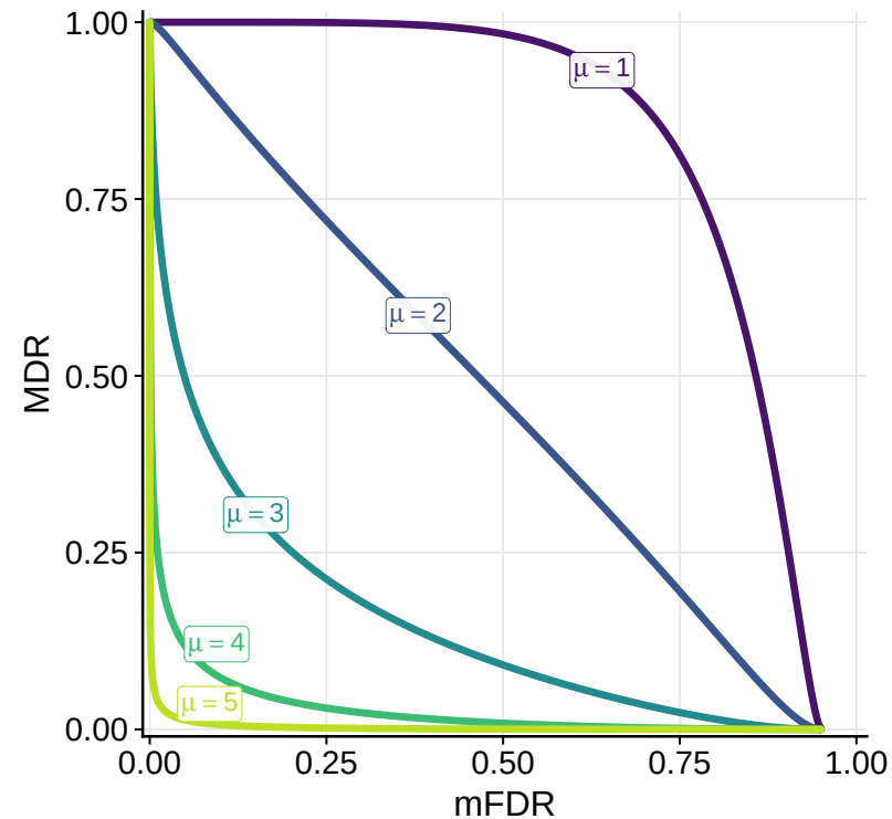
mFDR-MDR trade-off ( \pi = 0.05 )
