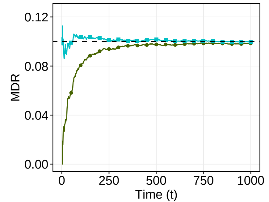
(b.2) Surge signal proportion
