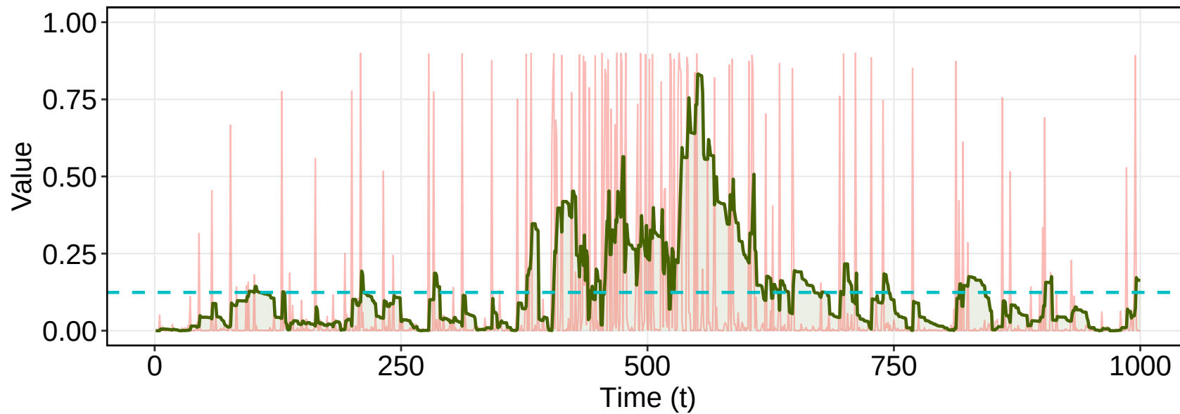
(b.1) Gaussian surge signal proportion: \pi_t rises from 0.05 to 0.3 and returns
