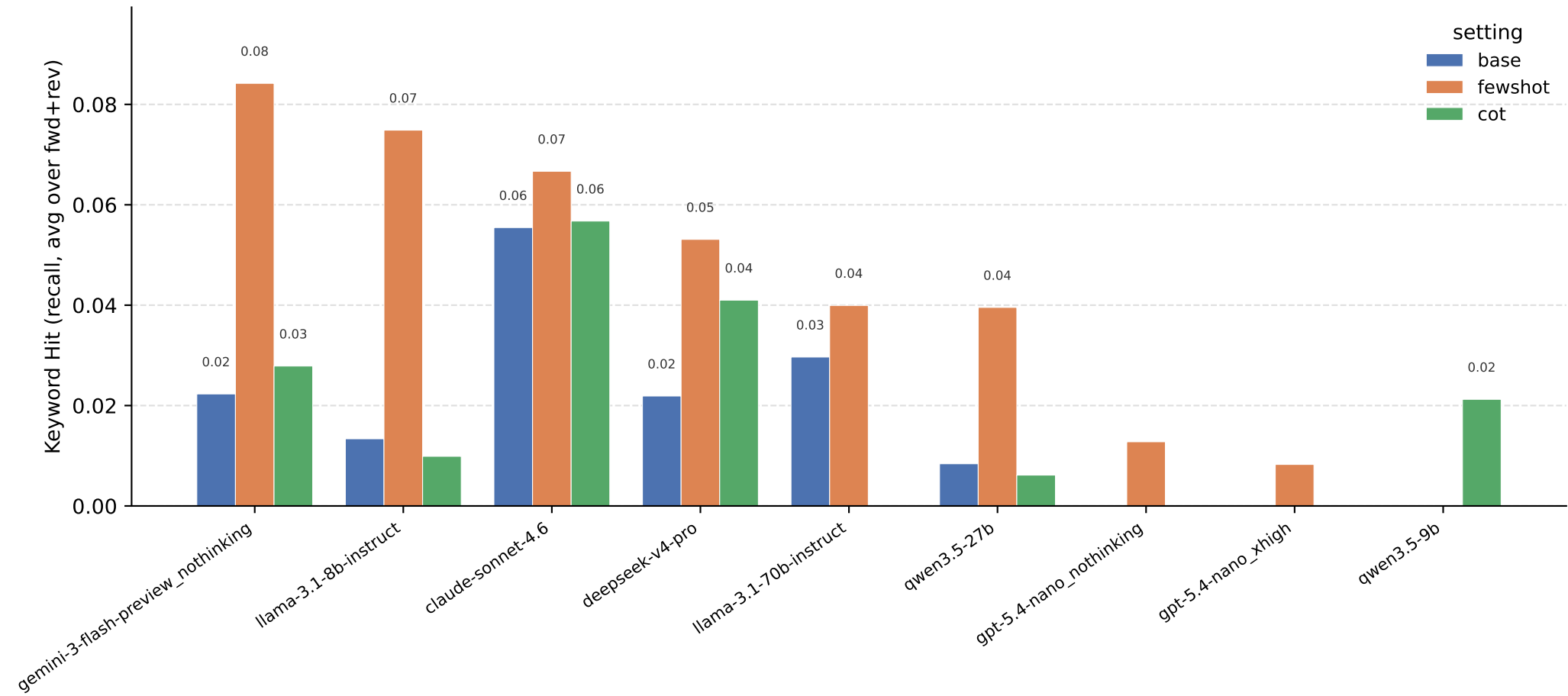
Task 3: Keyword Hit across models × prompting settings
