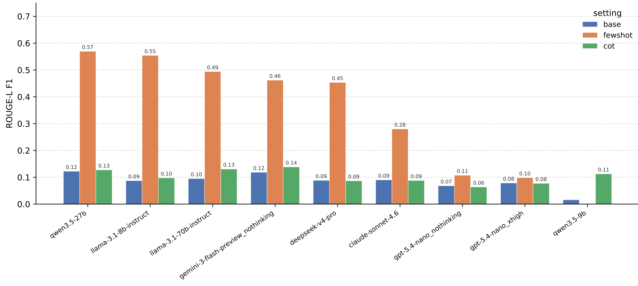
Task 3: ROUGE-L F1 across models × prompting settings
