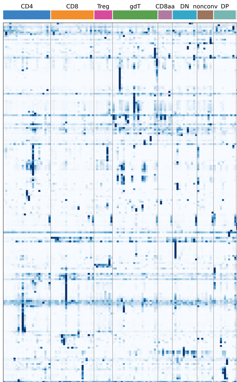
EBMF factors
