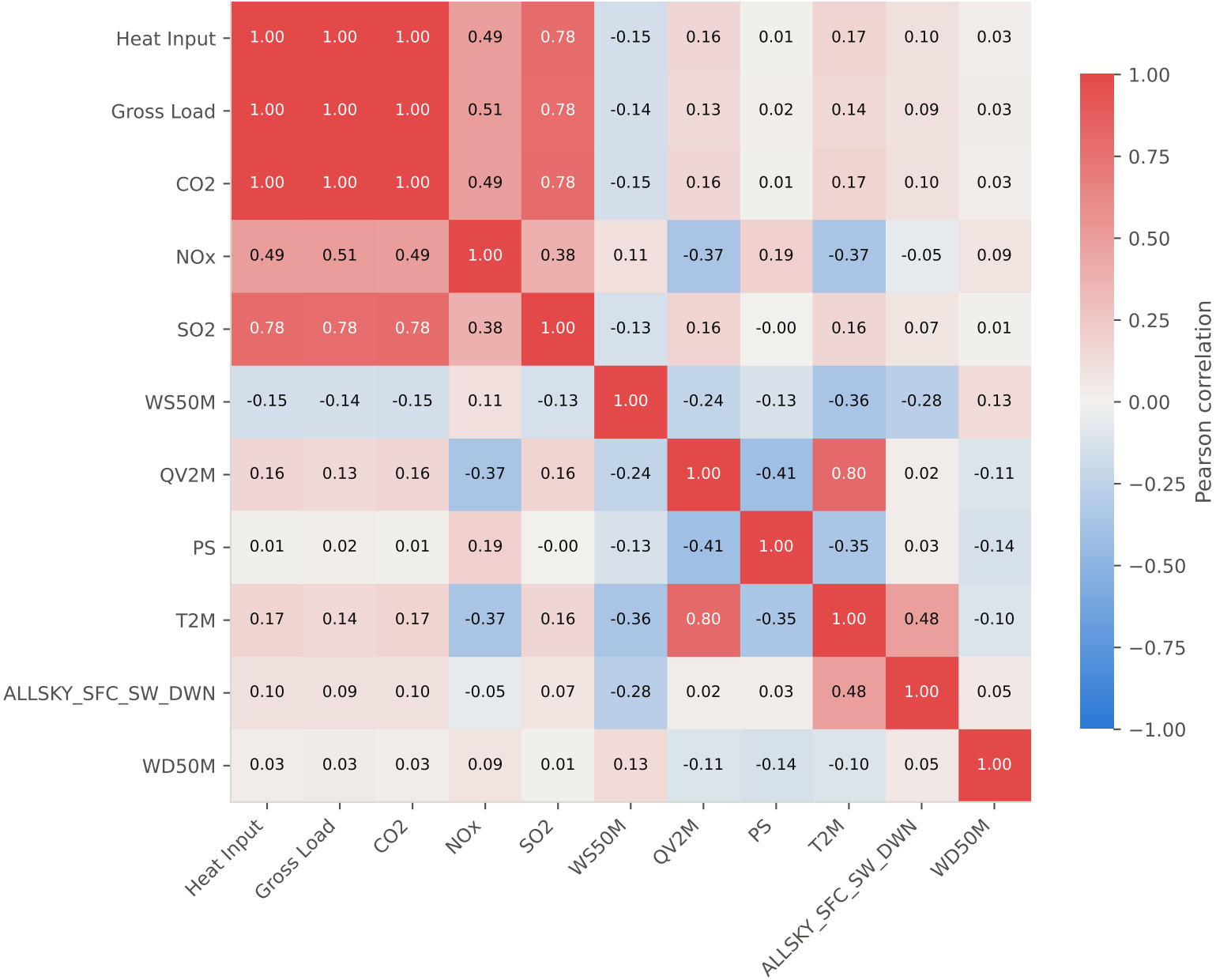
Correlation between plant variables and weather (operating hours only)
