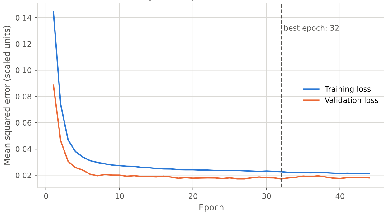
Transformer training history — CO2 Mass (short tons)
