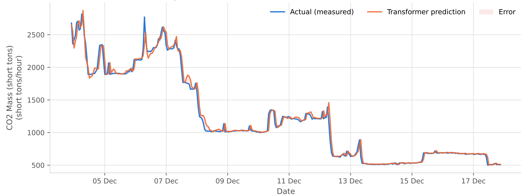
Transformer: first 14 days of the test set — CO2 Mass (short tons)
