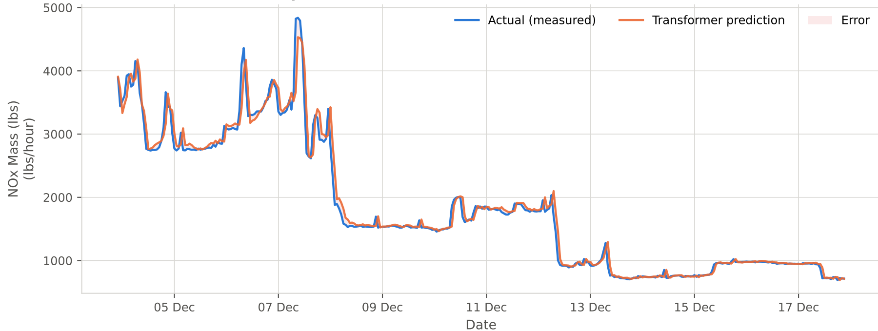
Transformer: first 14 days of the test set — NOx Mass (lbs)
