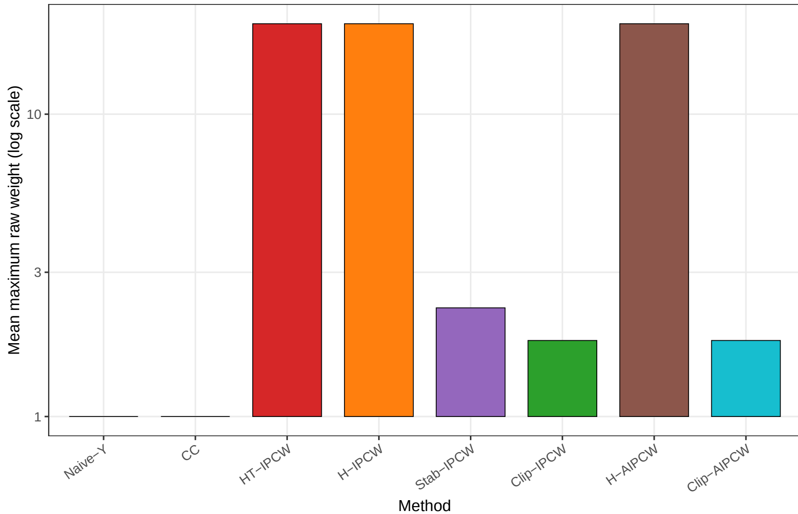
GBSG real-data application: maximum inverse-censoring weights
