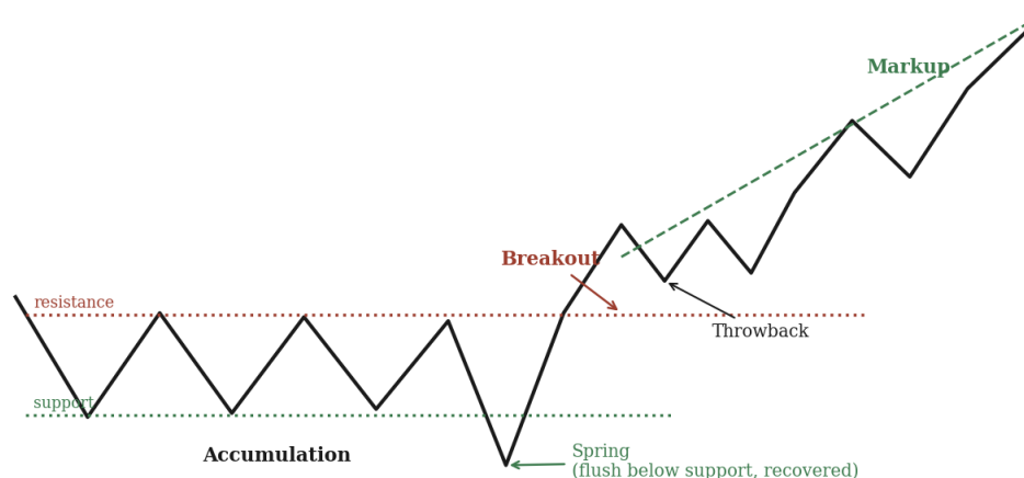
The Wyckoff template: accumulation, spring, breakout, markup (schematic)
