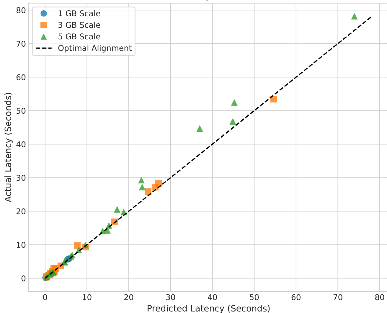
GreenQO Latency Across Volumes
