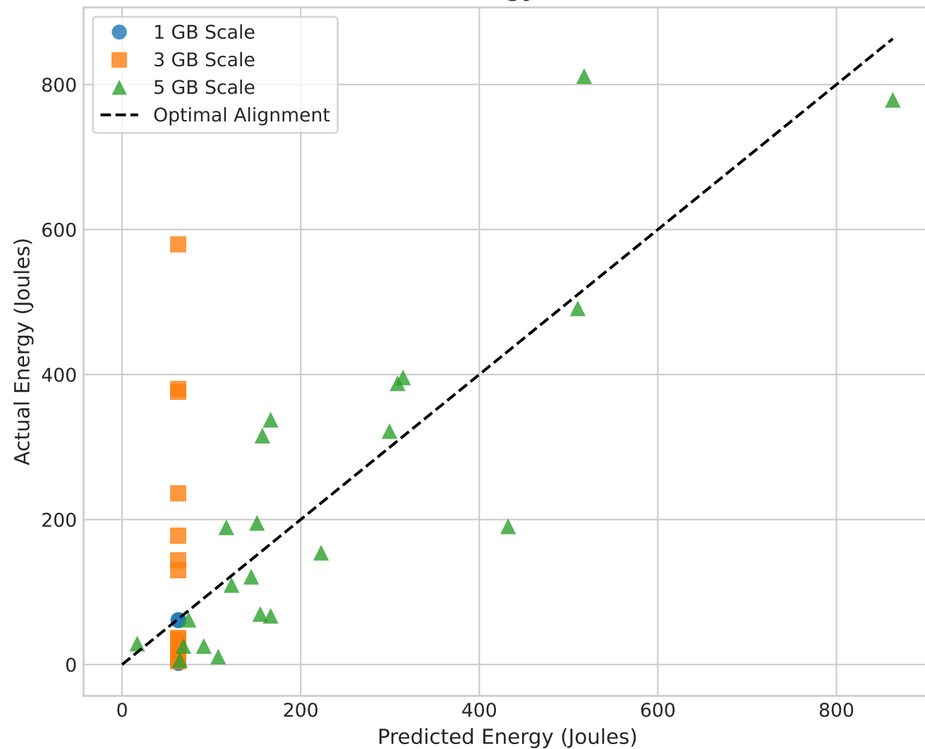
Baseline MLP Energy Across Volumes
