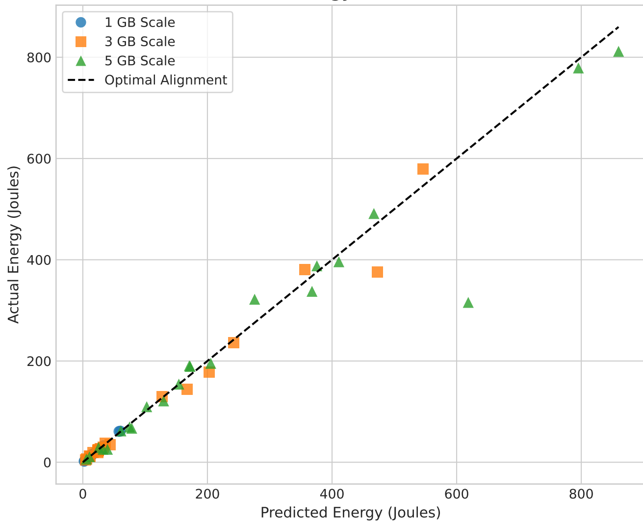
GreenQO Energy Across Volumes
