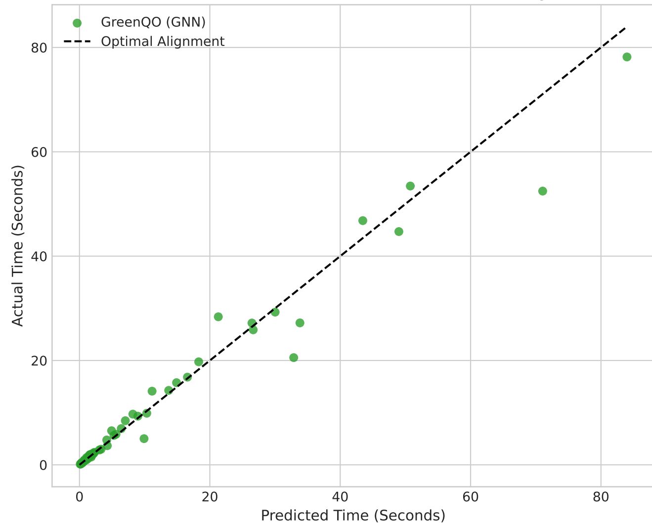
GreenQO GNN: Predicted vs. Actual Latency
