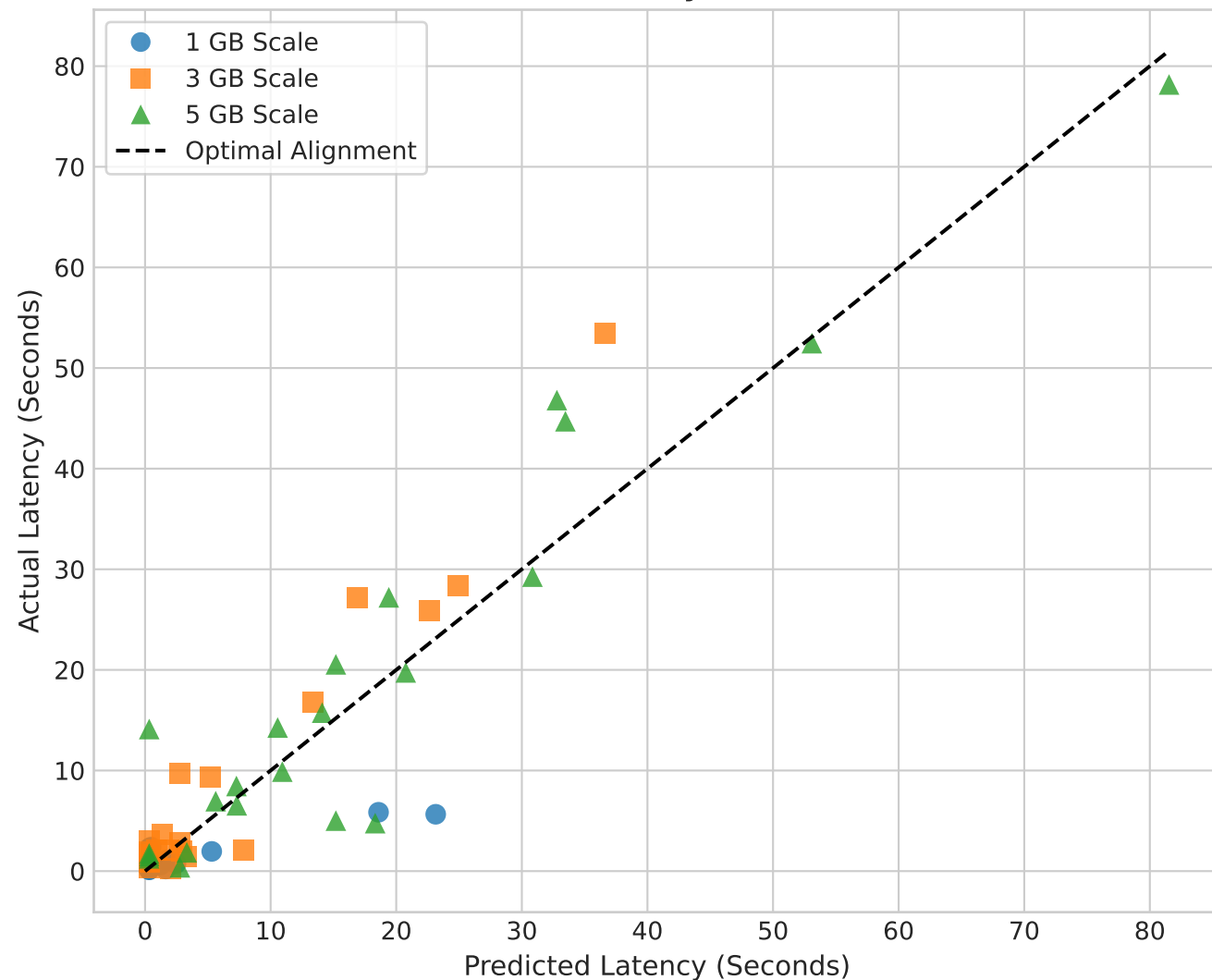
Baseline MLP Latency Across Volumes
