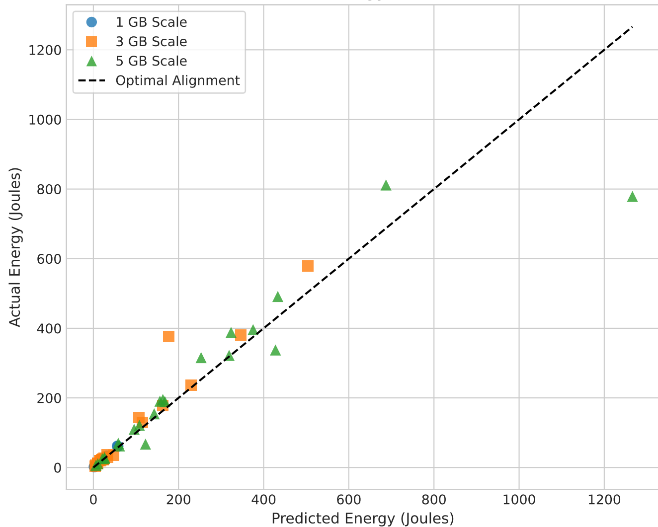
GreenQO GNN Energy Across Volumes
