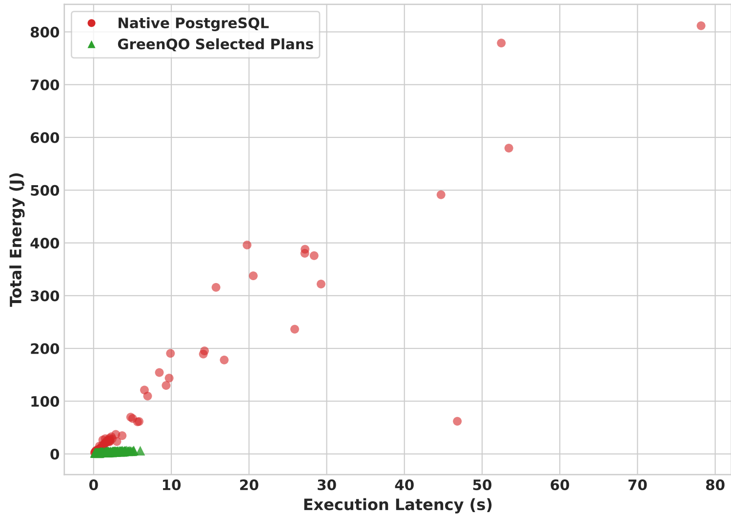
Latency vs. Total Energy Consumption
