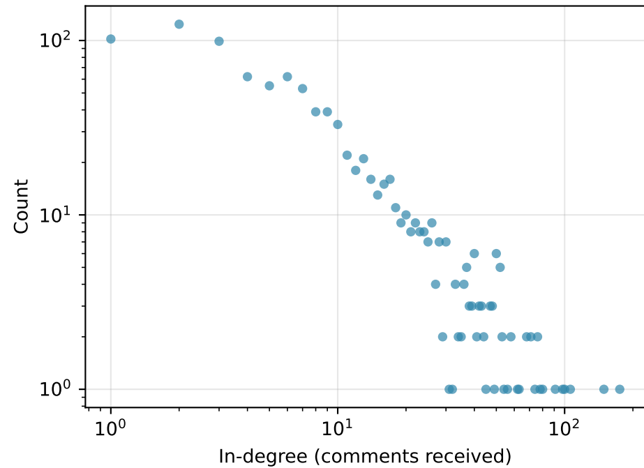
In-Degree Distribution
