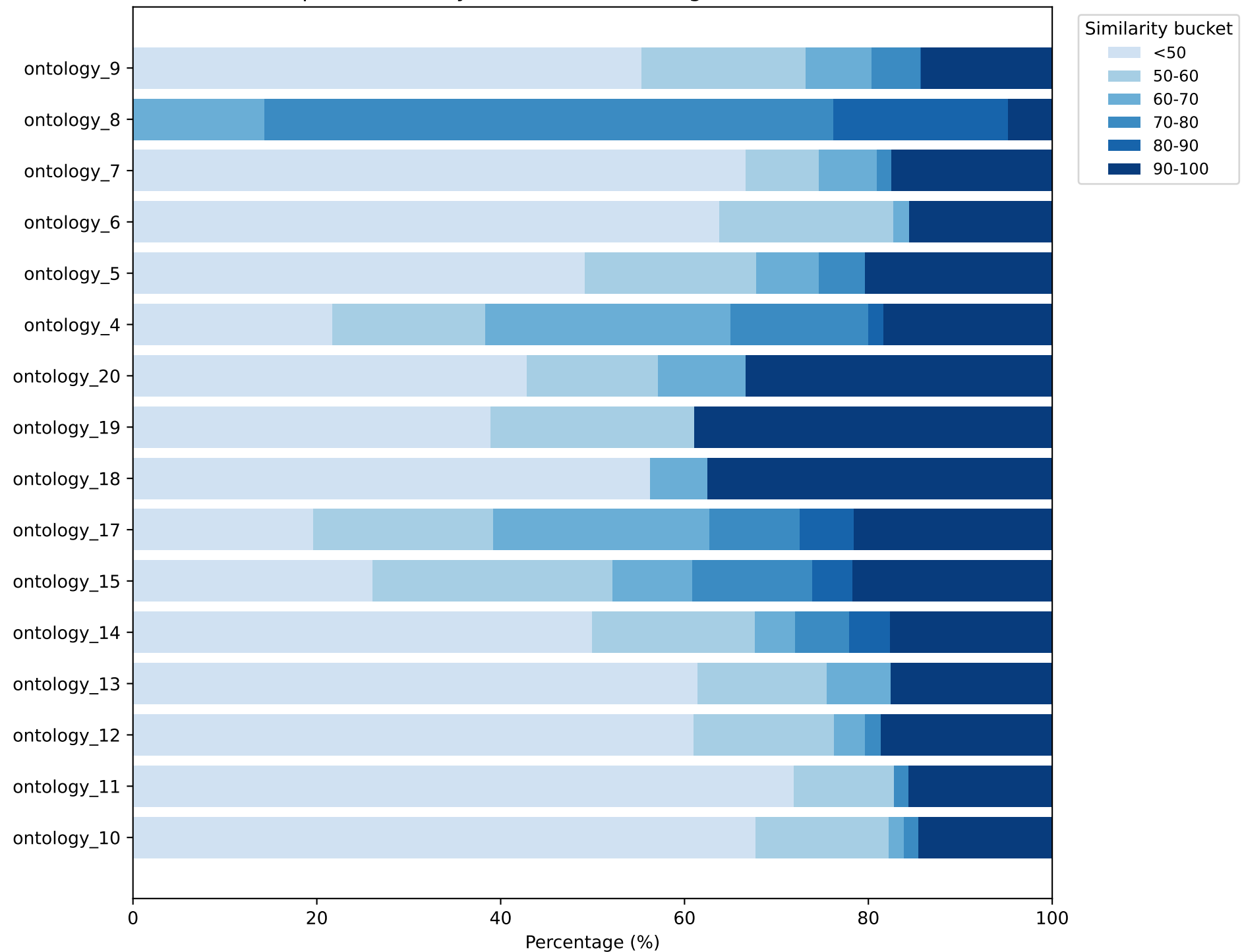
GPT-5 AquaDiva: Entity-Level Semantic Alignment vs Gold Standard
