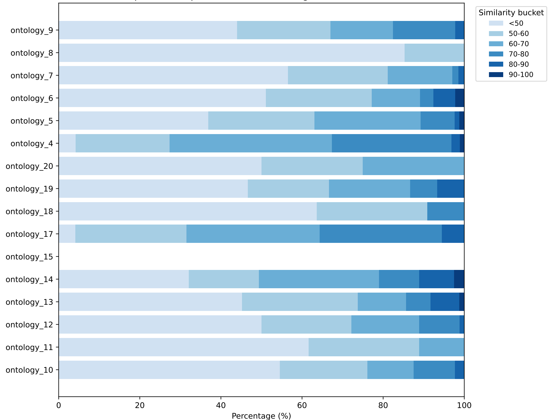
GPT-5 AquaDiva: Triple-Level Semantic Alignment vs Gold Standard
