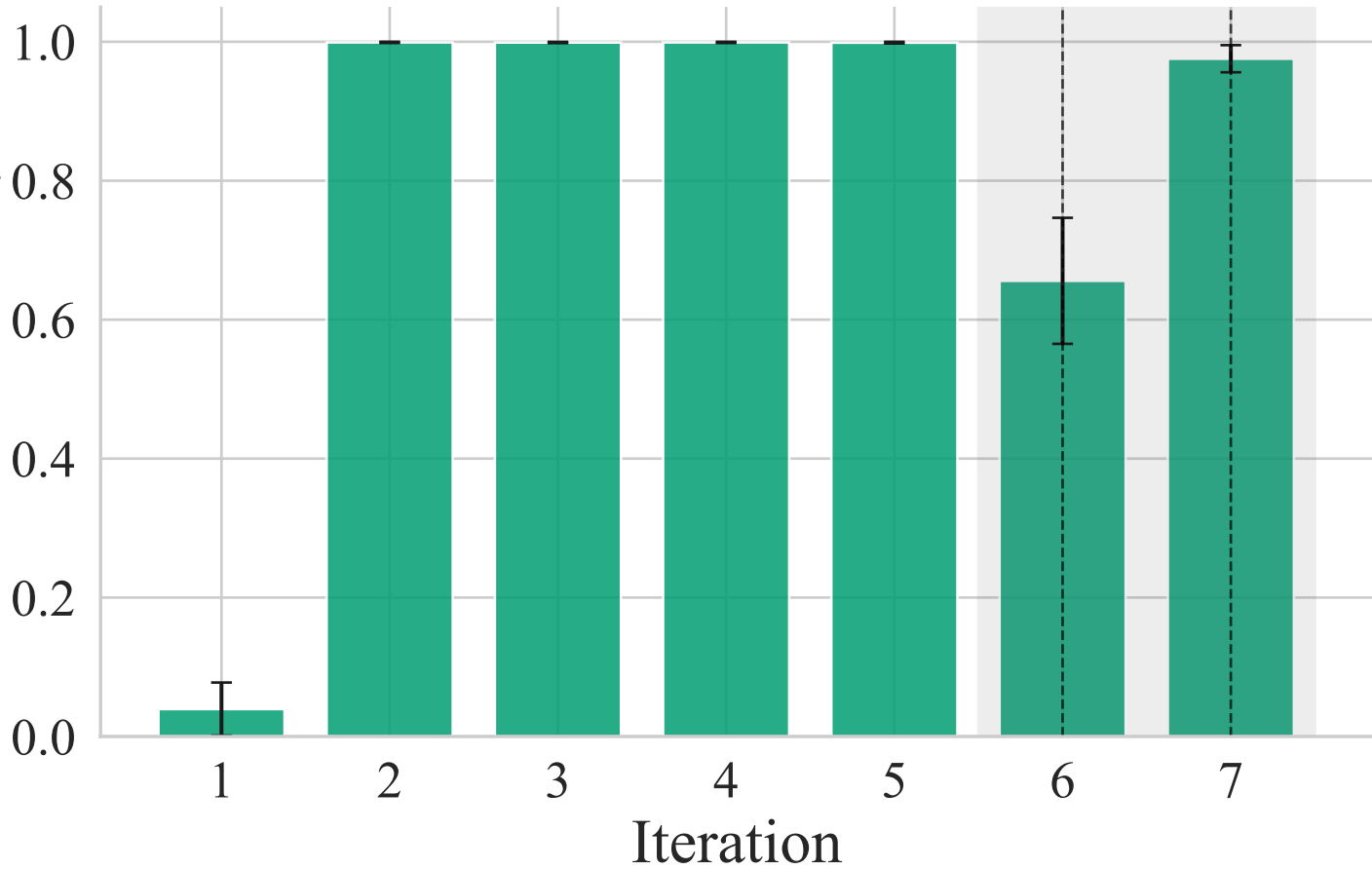
Cosine Similarity
