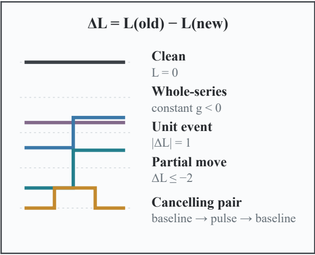
a Lag-state dictionary
