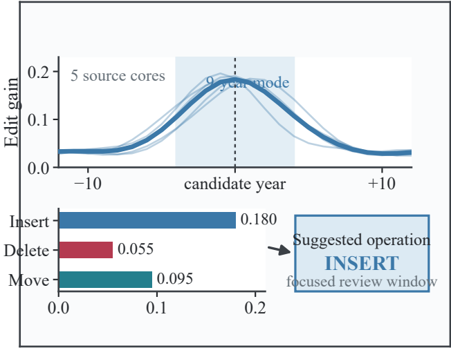
f Counterfactual and multi-reference consensus
