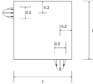
FIGURE 5.7: Current curved benchmark schematic from the working code base. If the Bayat–Li–Alexandersen pipe-bend or U-bend is adopted for the final Chapter 5 campaign, this figure should be replaced by the corresponding updated geometry and boundary-condition definition.
