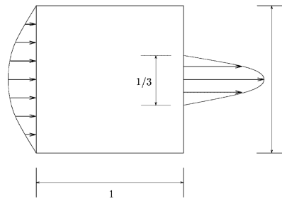
FIGURE 5.1: Current diffuser benchmark geometry and boundary-condition layout. This figure can be retained for the final manuscript unless the diffuser definition itself is modified.
