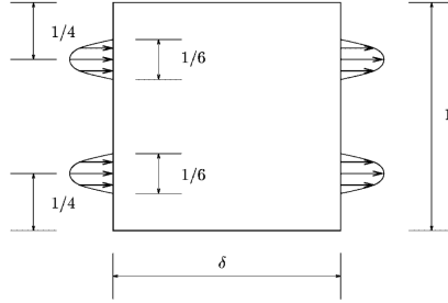
FIGURE 5.4: Current double-pipe benchmark geometry and boundary-condition layout.
