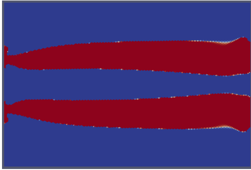
(A) Current final projected topology from FEniCS-SA.
