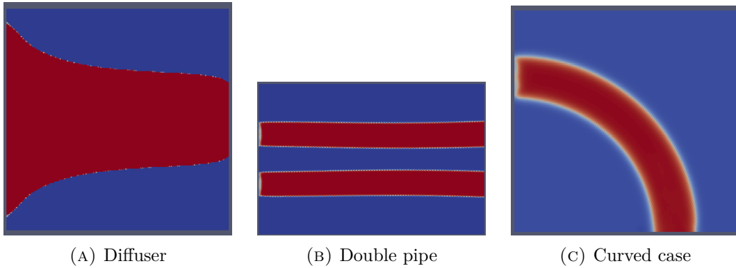
FIGURE 5.10: Current semi-frozen topologies. These results should be interpreted as exploratory only. Before claiming any superiority over the frozen adjoint, the final study should introduce non-design inlet and outlet regions and use turbulent boundary conditions that do not inject artificial shear singularities at the design boundary.
