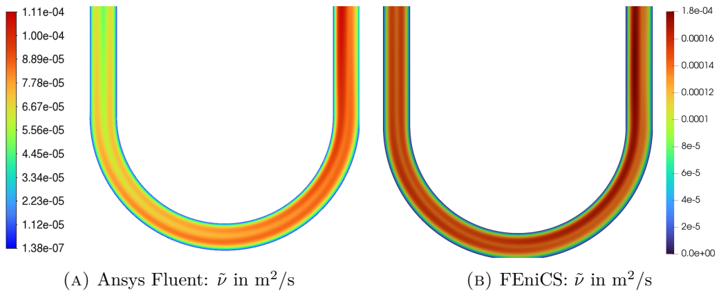
FIGURE 4.6: U-bend modified turbulent viscosity.
