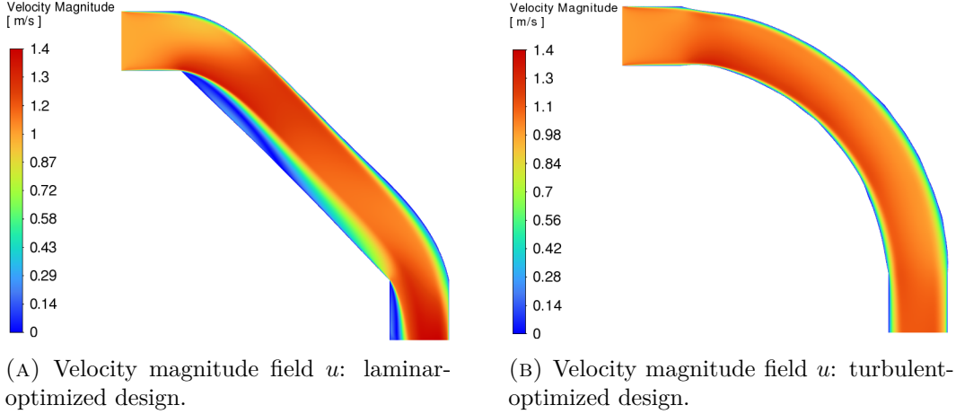
FIGURE 6.4: Velocity-contour comparison for the extracted pipe-bend designs under identical turbulent operating conditions (SST k - \omega model).
