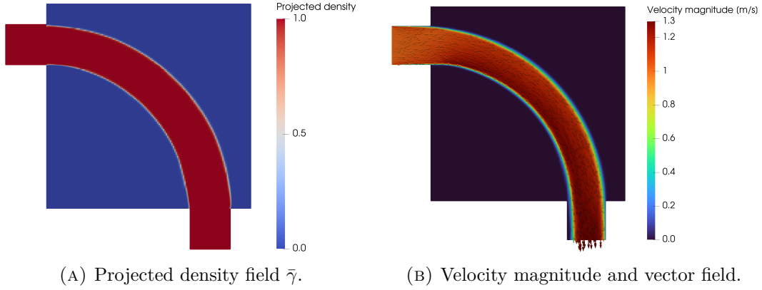
FIGURE 6.2: FEniCS-SA optimization result for the pipe-bend benchmark at V_f = 0.25 . Final objective value J_p = 0.2130 Pa.
