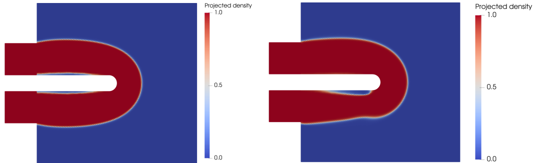
(A) Projected density field \bar{\gamma} : laminar-optimized design ( Re = 1 ).
