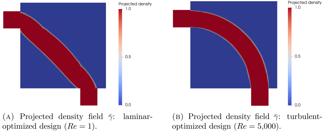
FIGURE 6.3: Laminar and turbulent topology comparison for the pipe-bend benchmark.
