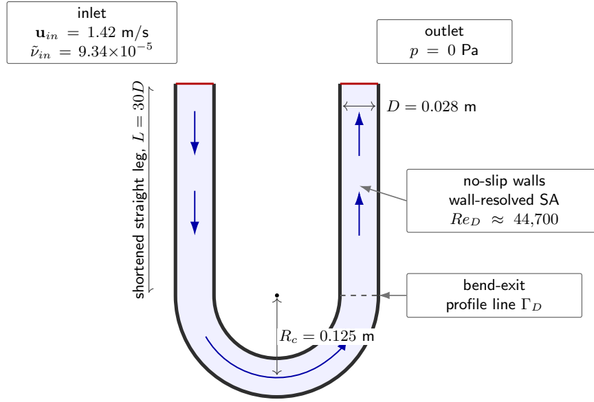
FIGURE 4.4: Shortened 2D U-bend verification setup (ChatGPT, 2026).
