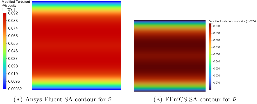
FIGURE 4.3: Modified turbulent viscosity (SA transport variable) for the 2D channel benchmark.
