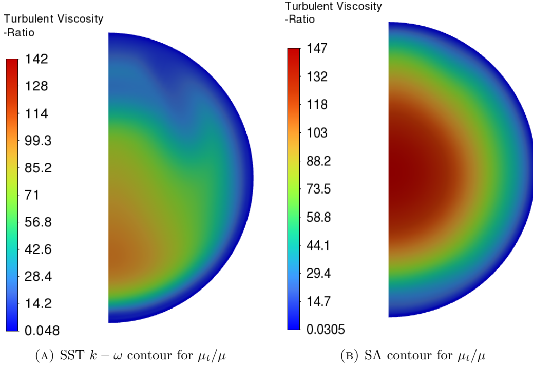
FIGURE 2.8: Turbulent viscosity ratios for the U-bend. The SA model overpredicts turbulent viscosity.
