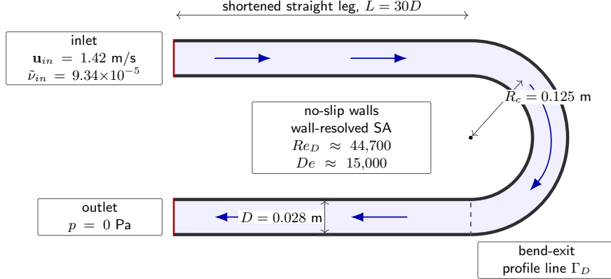
FIGURE 4.4: Schematic of the shortened 2D U-bend verification setup based on the VMFL048 operating point from the Ansys verification manual [8]. The profile line \Gamma_D is used for the bend-exit velocity comparison.
