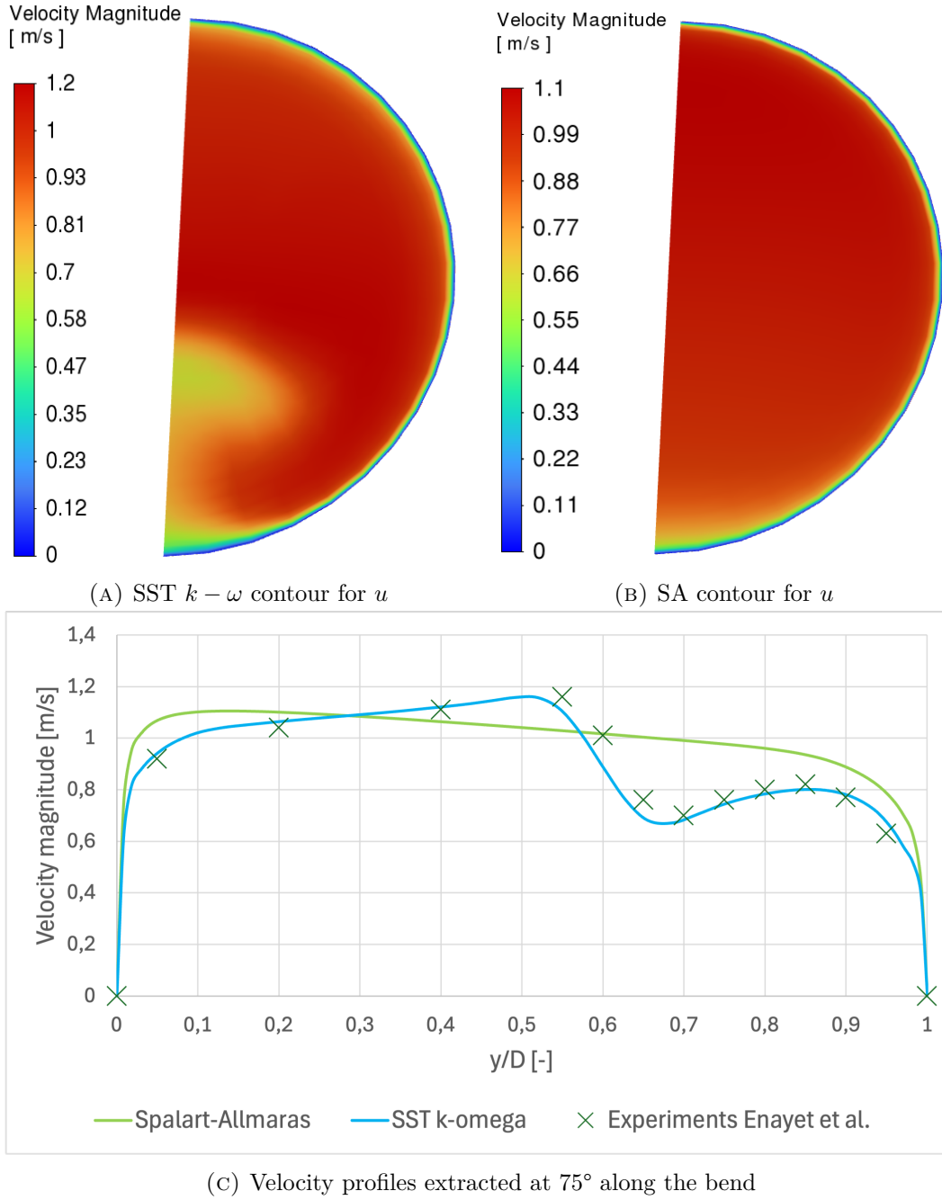
FIGURE 2.10: Flow predictions at the 75° plane along the 90° pipe bend ( R_c = 2.8D , Re_D \approx 43,000 , De \approx 18,000 ). The SA model over-smooths the velocity gradients near the inner wall, deviating from both the SST k - \omega model and the experimental data from Enayet et al. [22].
