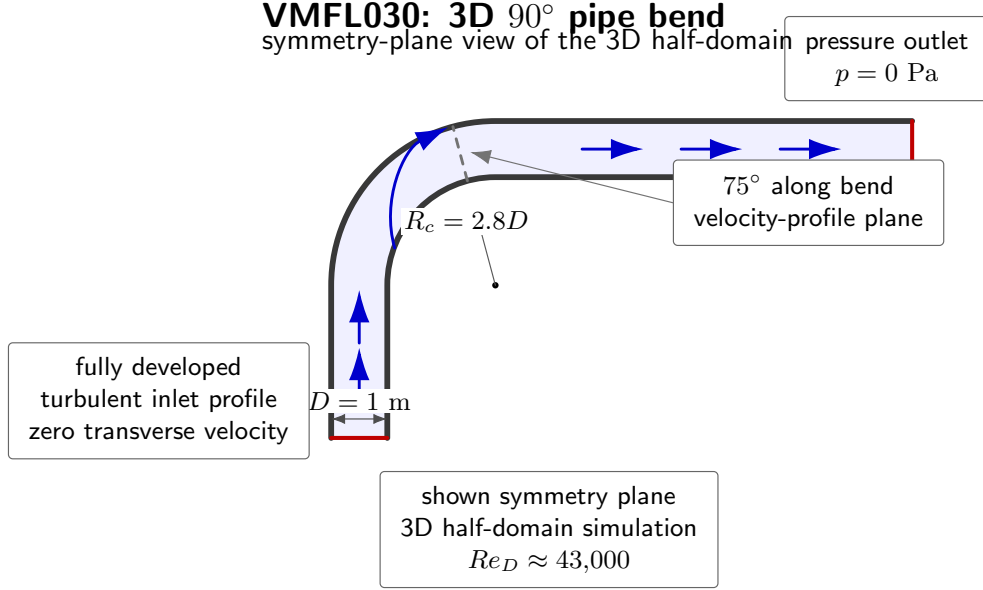
FIGURE 2.9: Geometry and boundary conditions for the VMFL030 3D 90° pipe-bend benchmark adopted from the Ansys Fluid Dynamics Verification Manual [8]. The schematic is not to scale.
