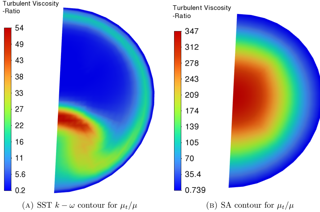
FIGURE 2.11: Turbulent viscosity ratios for the 90° pipe bend. The SA model massively overpredicts turbulent viscosity.
