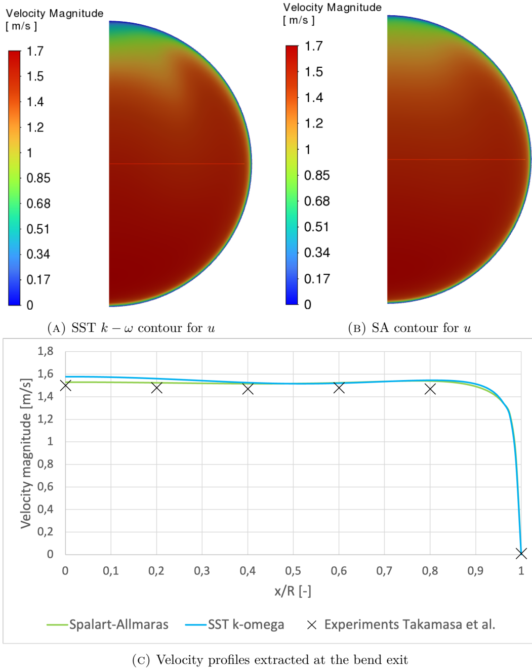
FIGURE 2.7: Flow predictions for a 180° U-bend ( R_c \approx 4.46D , Re_D \approx 44,700 , De \approx 15,000 ). The SA model matches the SST k - \omega contours and aligns with the experimental data from Takamasa and Kondo [55].
