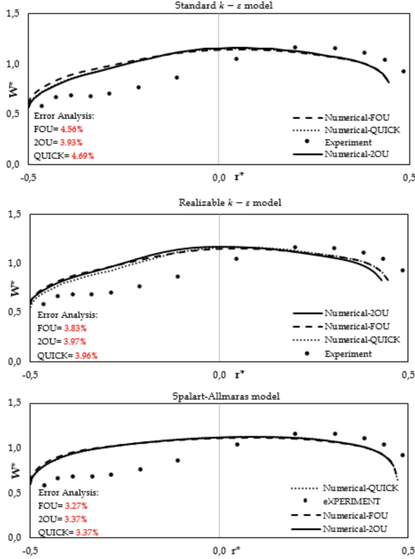
FIGURE 2.1: Streamwise velocity profiles in a 90^\circ pipe bend ( R_c = 7D , Re_D \approx 34,000 , De \approx 9,000 ). The SA model performs relatively well for mild curvature. Reprinted from Apalowo [8].
