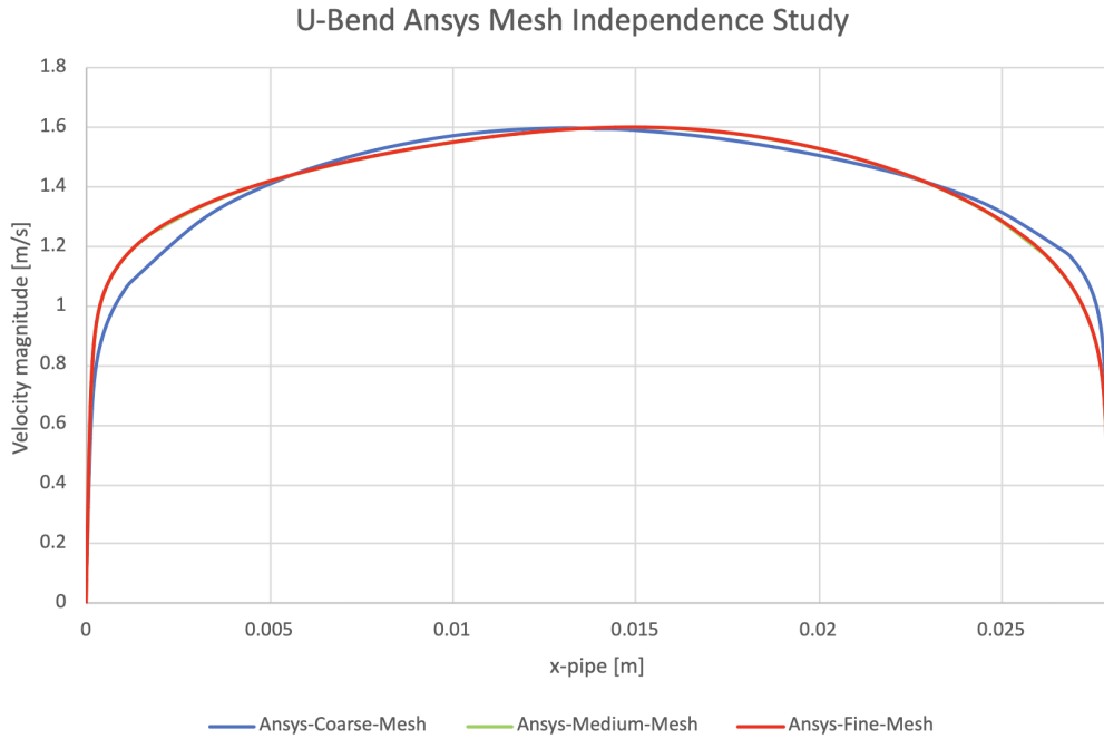
FIGURE A.4: Velocity profiles at the U-bend exit, extracted across the pipe diameter D = 0.028 m, for the Coarse, Medium, and Fine Ansys grids, demonstrating spatial convergence of the commercial baseline.
