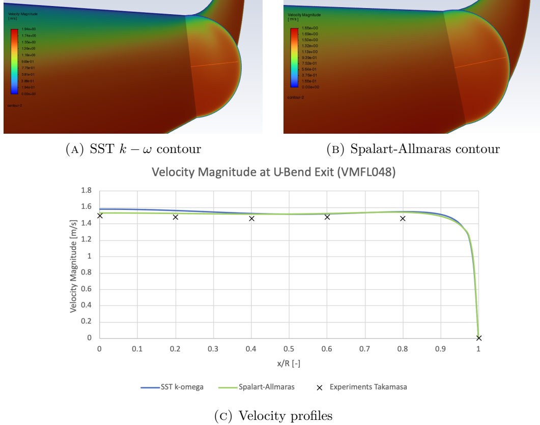
FIGURE 2.3: Flow predictions for a 180^\circ U-bend ( R_c \approx 4.46D , Re_D \approx 44,700 , De \approx 15,000 ). The SA model matches the SST k - \omega contours and aligns with the experimental data from Takamasa and Kondo [48].
