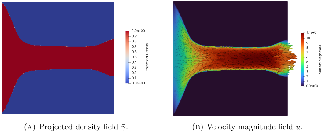
FIGURE 6.12: FEniCS-SA optimization result for the diffuser benchmark at V_f = 0.30 . Final objective function value J_D = 2.8264 \times 10^5 W/m.
