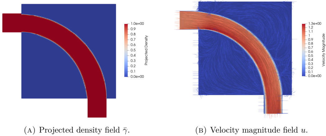
FIGURE 6.2: FEniCS-SA optimization result for the pipe-bend benchmark at V_f = 0.25 . Final objective function value J_p = 0.2032 Pa.
