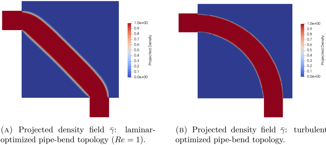
FIGURE 6.4: Laminar and turbulent topology comparison for the pipe-bend benchmark.
