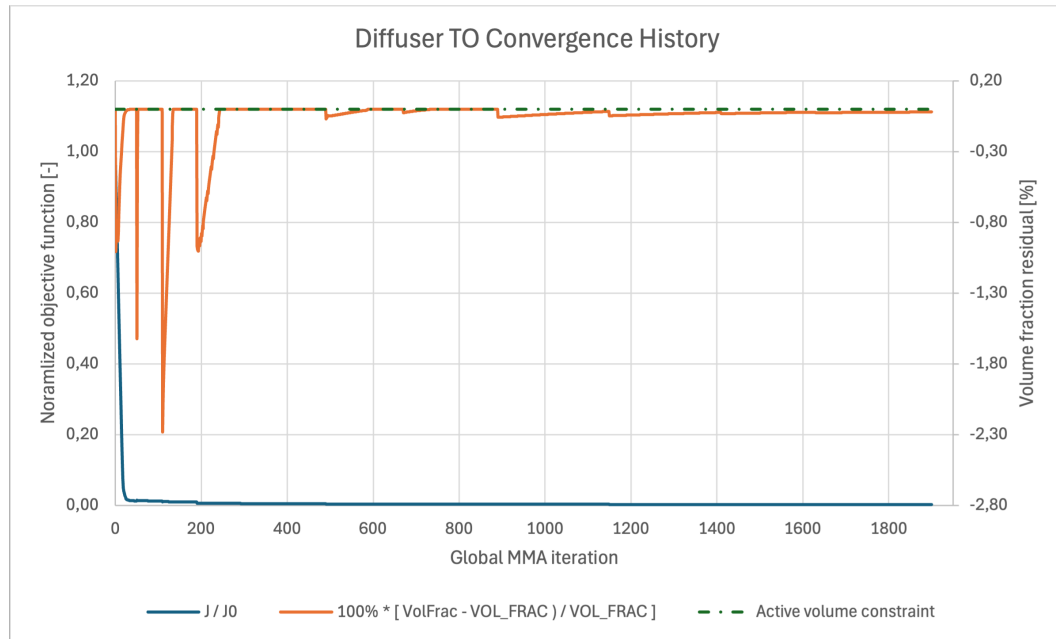
FIGURE 6.13: Optimization convergence history for the diffuser benchmark. The final figure should use a combined dissipation-objective and volume-residual plot.
