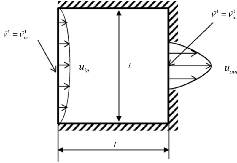
FIGURE 6.11: Geometry and boundary conditions for the diffuser benchmark from Yoon [55].
