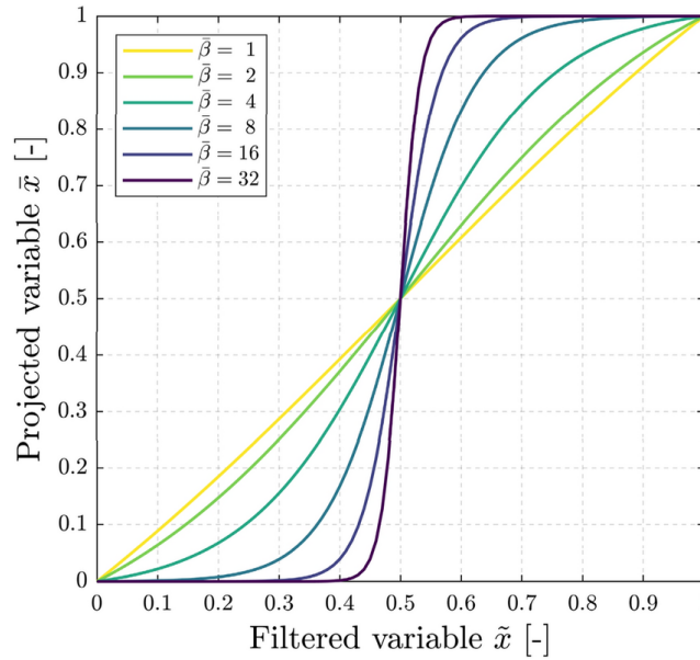
FIGURE 4.2: Heaviside projection from Eq. 4.18 at \eta = 0.5 for \beta = \{1, 2, 4, 8, 16, 32\} , reproduced from Ooms et al. [34].
