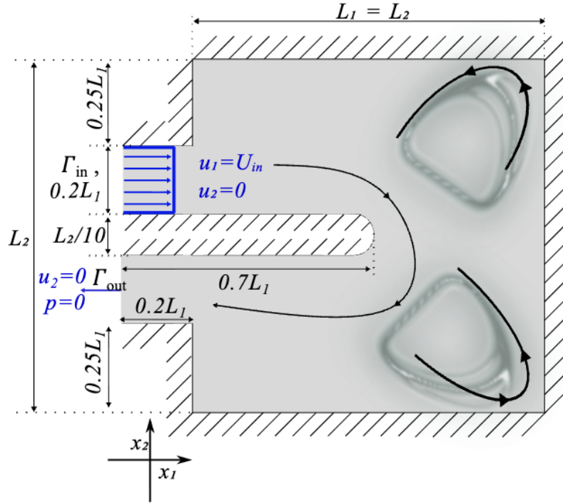
FIGURE 6.6: Geometry and boundary conditions for the U-bend benchmark from Bayat et al. [11].
