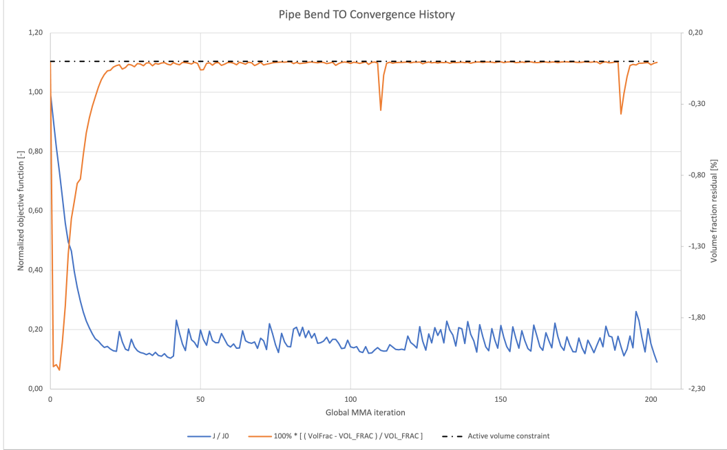
FIGURE 6.3: Optimization convergence history for the pipe-bend benchmark. The blue curve shows the normalized pressure objective J/J_0 , while the orange curve shows the relative volume-fraction residual r_V from Eq. (6.4).
