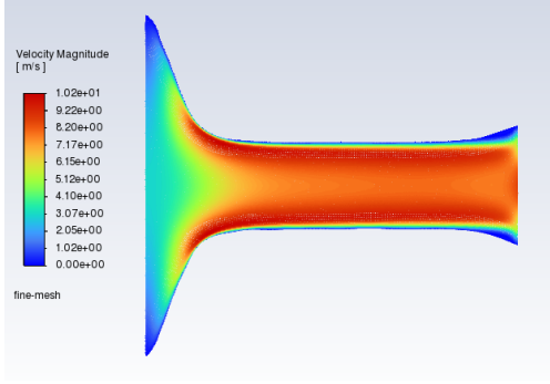
(A) Velocity magnitude field u : laminar-optimized design.
