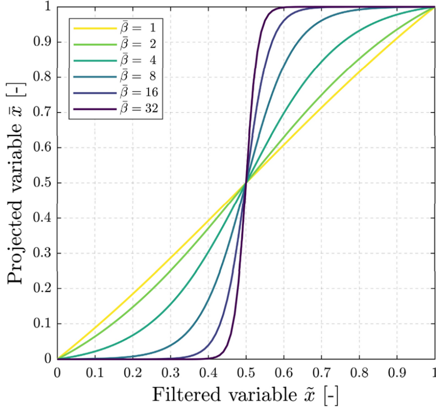
FIGURE 4.2: Heaviside projection from Eq. 4.18 at \eta = 0.5 for \beta = \{1, 2, 4, 8, 16, 32\} , ordered from smoothest to steepest. Increasing \beta concentrates the transition around the threshold and reduces the gray interval in the projected field. Figure reproduced from Ooms et al. [34], who use the same threshold value for the projection scheme.
