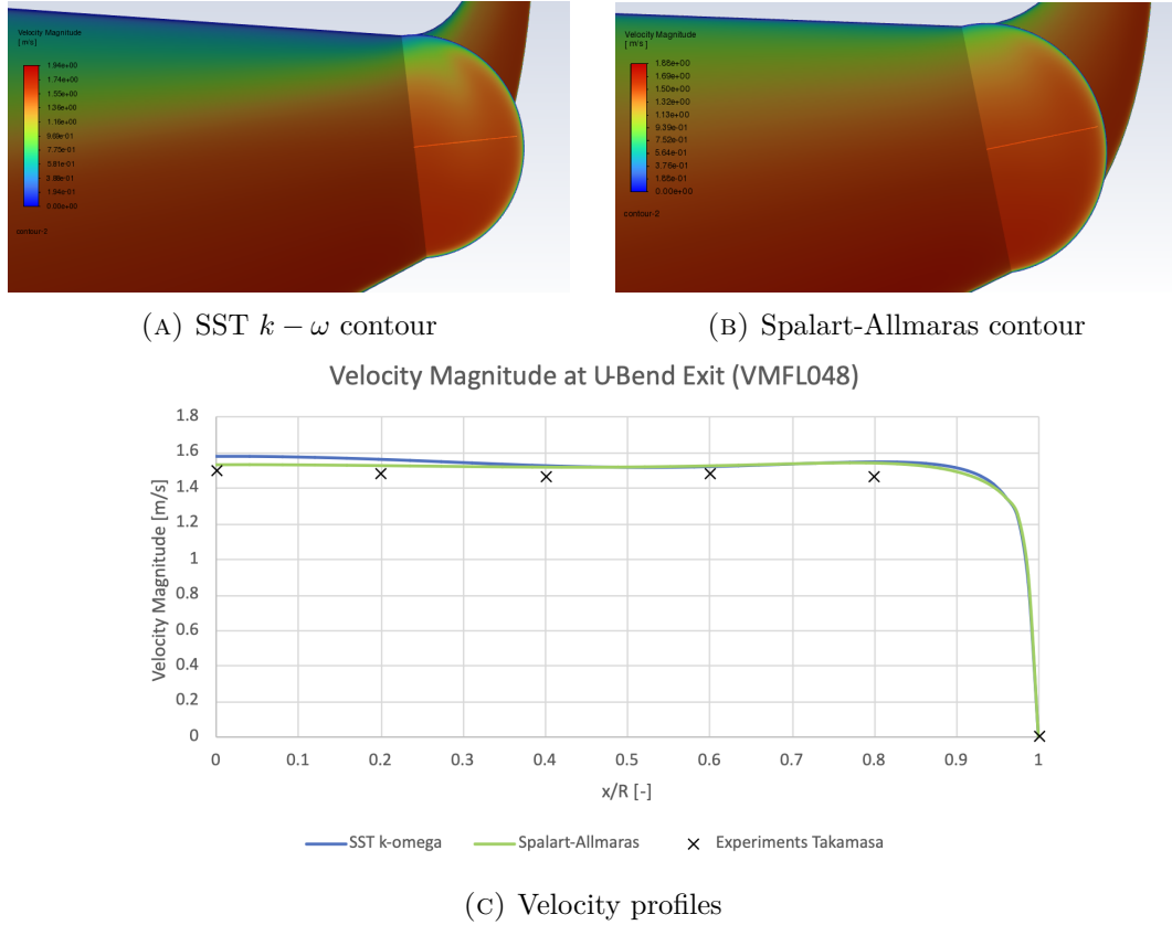
FIGURE 2.3: Flow predictions for a 180° U-bend ( R_c \approx 4.46D , Re_D \approx 44,700 , De \approx 15,000 ). The SA model matches the SST k - \omega contours and aligns with the experimental data from Takamasa and Kondo [48].
