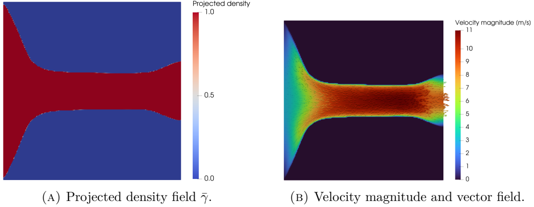
FIGURE 6.12: FEniCS-SA result for the velocity-outlet diffuser baseline at V_f = 0.30 . Final objective value J_D = 2.8264 \times 10^5 W/m.
