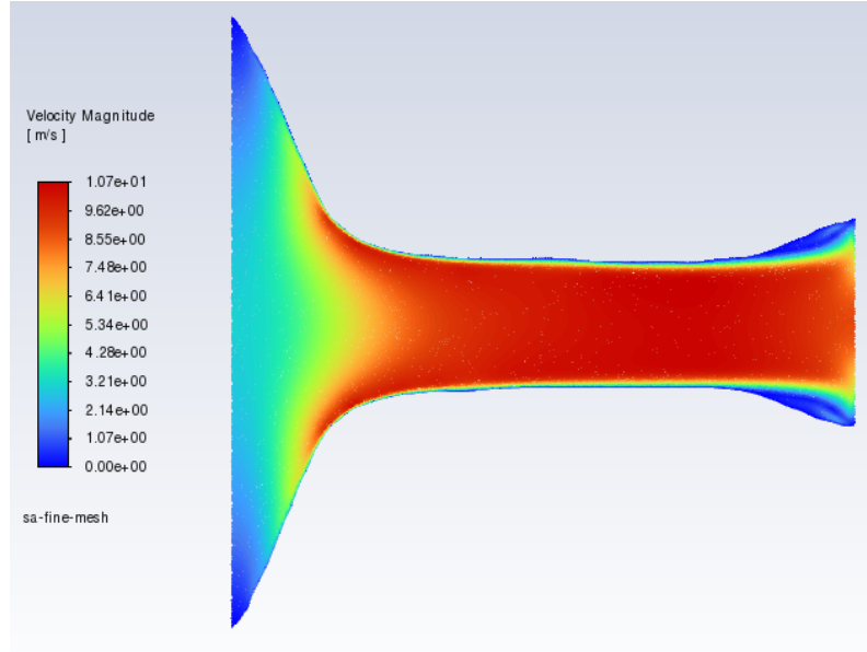
FIGURE 6.13: Ansys-SA velocity-magnitude contour for the extracted velocity-outlet diffuser baseline. The low-speed region near the widened outlet motivates the pressure-outlet sensitivity study.
