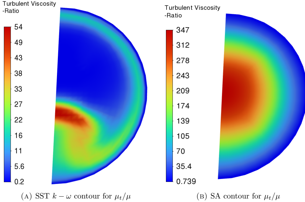
FIGURE 2.11: Turbulent-viscosity ratio contours for the VMFL030 90° pipe bend. Compared with SST k-\omega , SA predicts a much larger and more spatially uniform eddy-viscosity field across the section.
