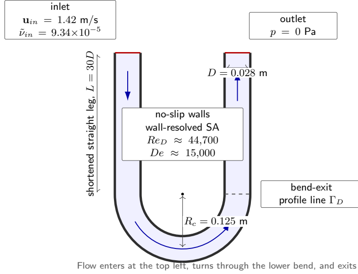
FIGURE 4.4: Schematic of the shortened 2D U-bend verification setup based on the VMFL048 operating point from the Ansys verification manual [8]. The U-bend is shown vertically: the flow enters at the top left, moves down the first straight section, turns through the lower bend, and leaves upward through the outlet leg at the top right. The profile line \Gamma_D is used for the bend-exit velocity comparison.
