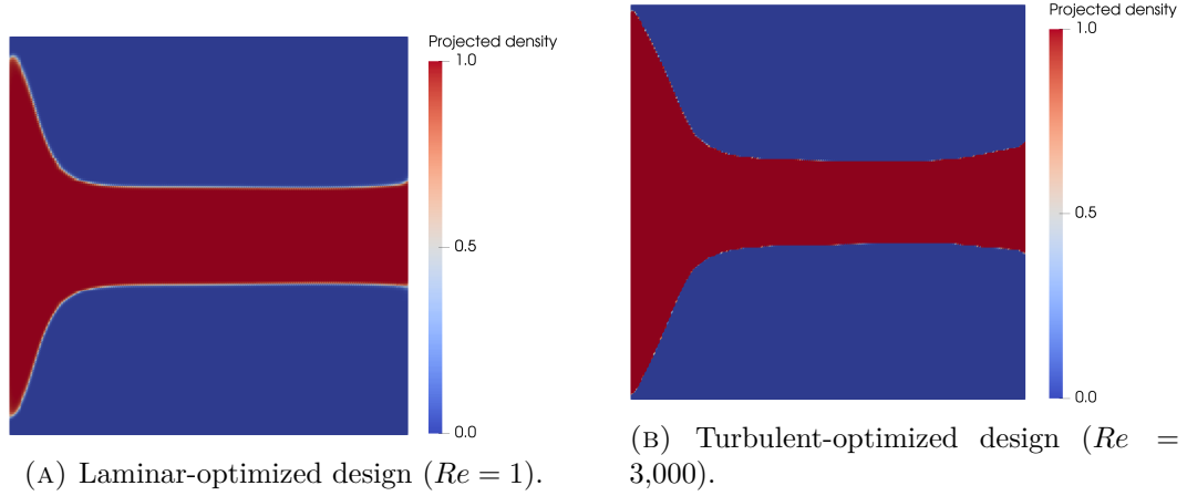
FIGURE 6.12: Laminar and turbulent topology comparison for the pressure-outlet diffuser benchmark.
