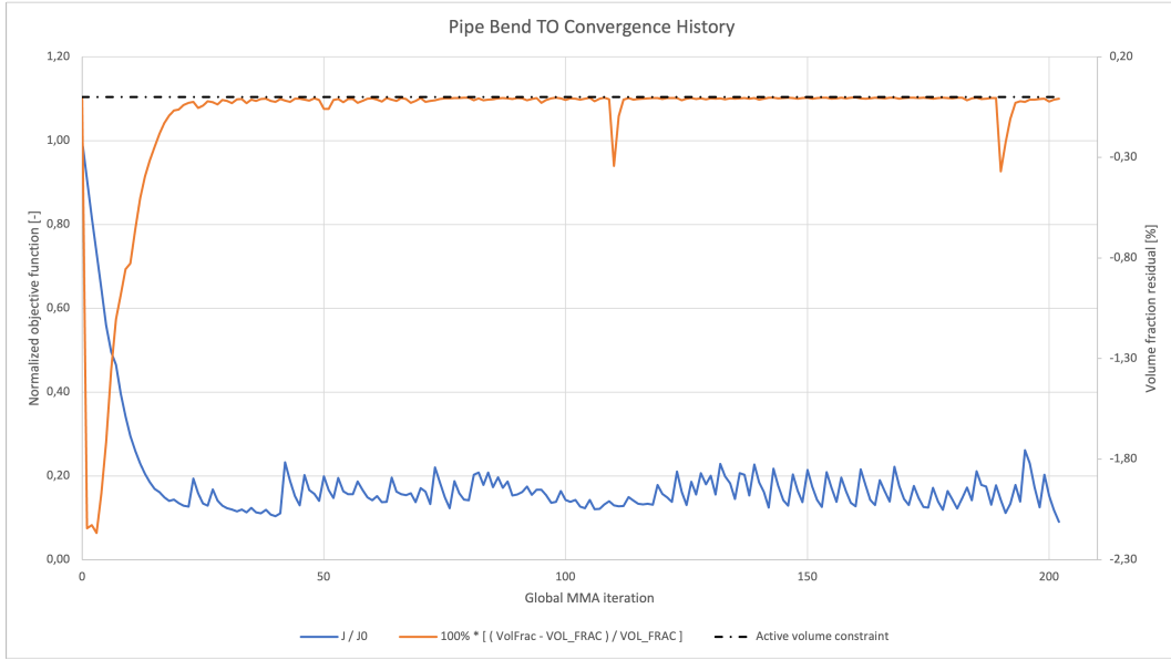
FIGURE C.1: Optimization convergence history for the turbulent pipe-bend benchmark. The blue curve shows the normalized pressure objective J/J_0 , while the orange curve shows the relative volume-fraction residual r_V from Eq. (C.3).
