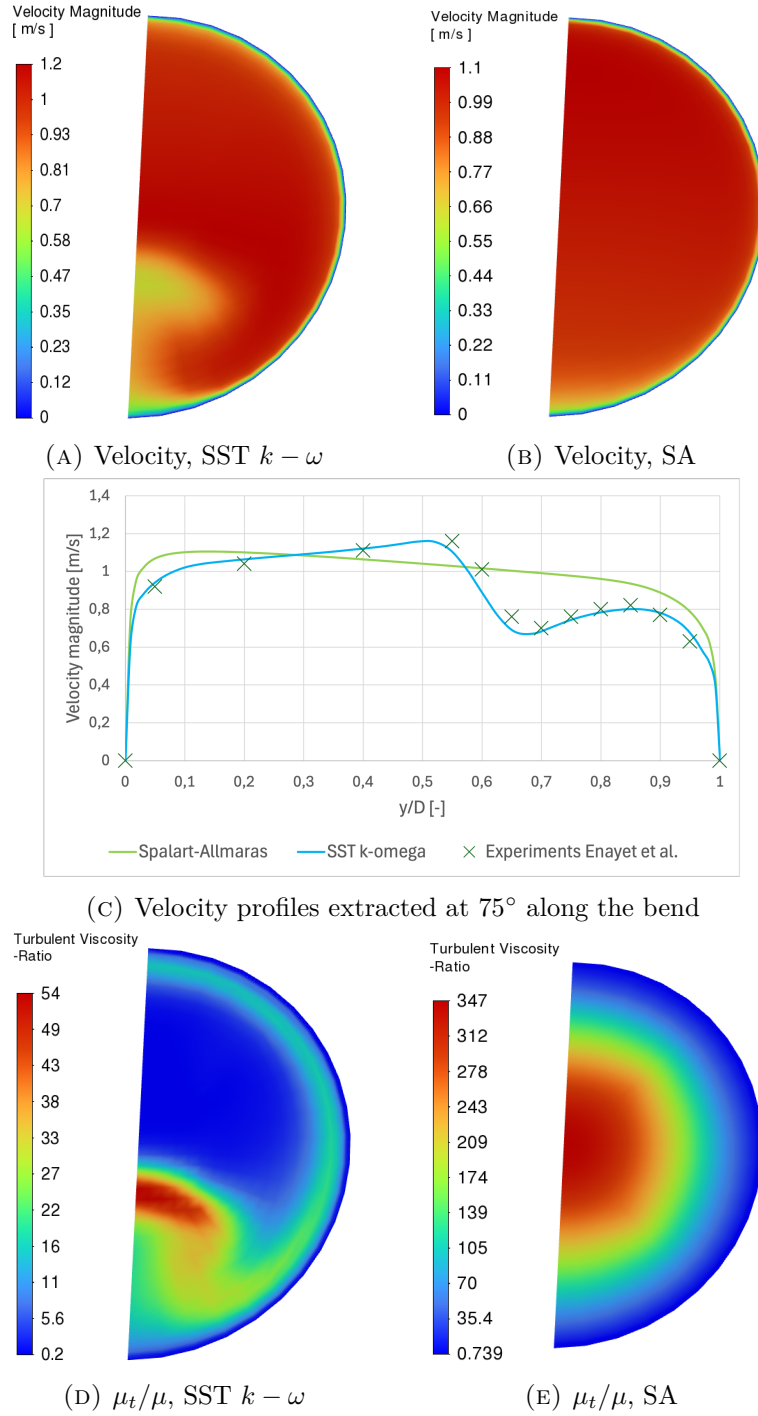
FIGURE 2.8: VMFL030 90^\circ pipe-bend RANS comparison: velocity contours, extracted velocity profile, and turbulent-viscosity ratio contours.
