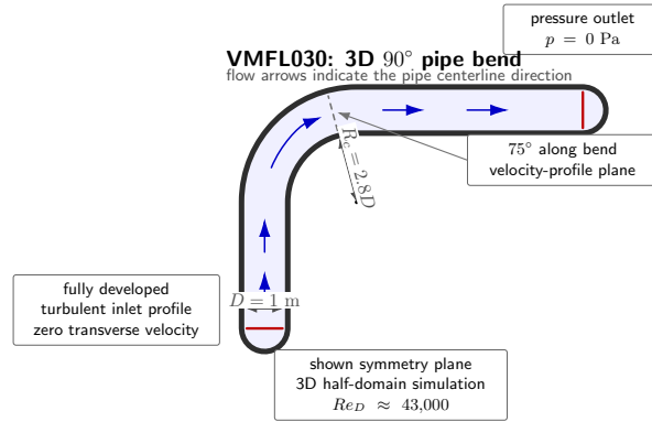
(B) VMFL030 3D 90° bend.
