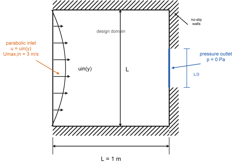
FIGURE 6.9: Geometry and boundary conditions for the pressure-outlet diffuser variant. The full-height inlet retains the shifted parabolic velocity profile, while the center-third outlet is assigned a fixed static pressure p = 0\text{ Pa} instead of a prescribed velocity profile.
