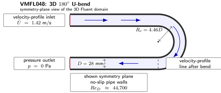
(A) VMFL048 3D U-bend.
