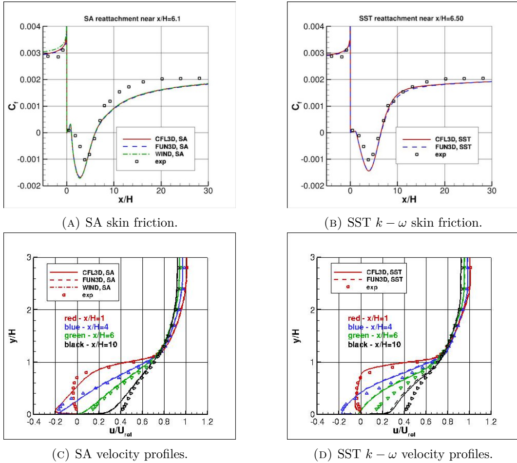
FIGURE 2.5: NASA Turbulence Modeling Resource comparison of SA and SST k - \omega predictions with the Driver-Seegmiller backward-facing-step experiment at Re_H \approx 36,000 [20, 38]. The velocity-profile comparison indicates better separated-flow recovery for SST k - \omega than for SA.
