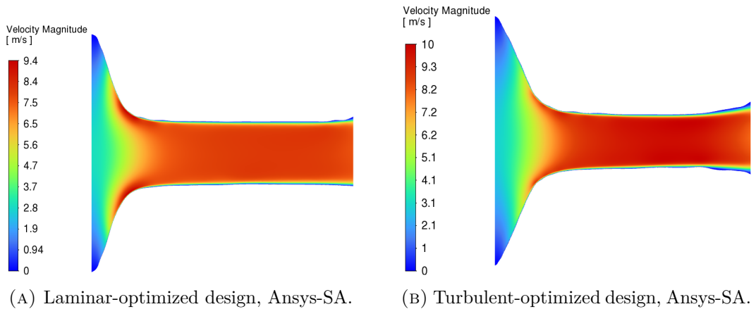
FIGURE 6.13: Ansys-SA velocity-magnitude comparison for the extracted pressure-outlet diffuser designs under identical turbulent operating conditions.
