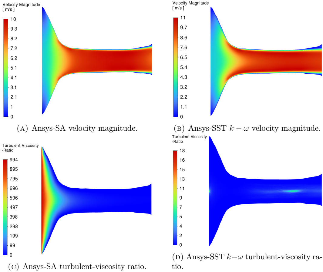
FIGURE 6.11: Closure diagnostics for the pressure-outlet turbulent diffuser. The velocity contours are similar enough that repeated full-domain velocity plots are not the main evidence; the turbulent-viscosity-ratio contours show the mechanism behind the much larger SA loss prediction.
