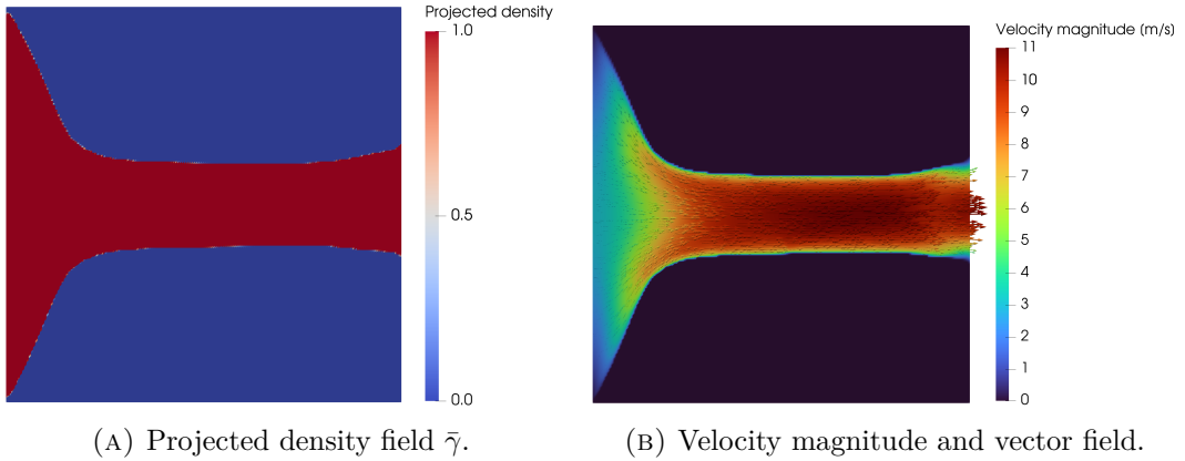
FIGURE 6.10: FEniCS-SA optimization result for the pressure-outlet diffuser at V_f = 0.30 . Final objective value J_D = 2.7664 \times 10^5\text{ W/m} .
