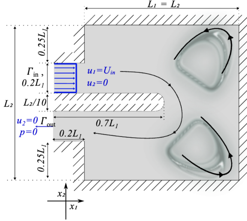
FIGURE 6.5: Geometry and boundary conditions for the U-bend benchmark from Bayat et al. [12].
