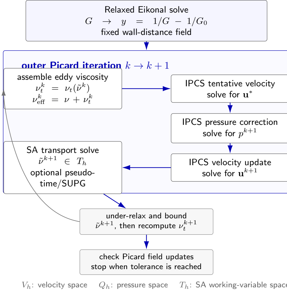
FIGURE 3.1: Nested Picard-IPCS coupling used by the FEniCS RANS-SA solver. The eddy viscosity \nu_t is assembled from the previous SA working variable \tilde{\nu} , the velocity-pressure pair is advanced by the IPCS weak problems, and the updated velocity then drives the next SA transport solve.
