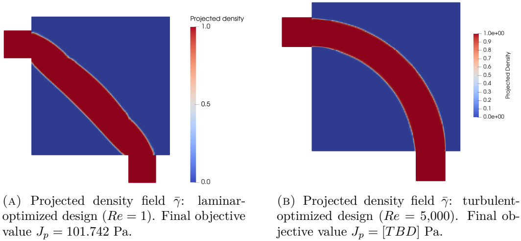
FIGURE 6.3: Laminar and turbulent topology comparison for the pipe-bend benchmark.
