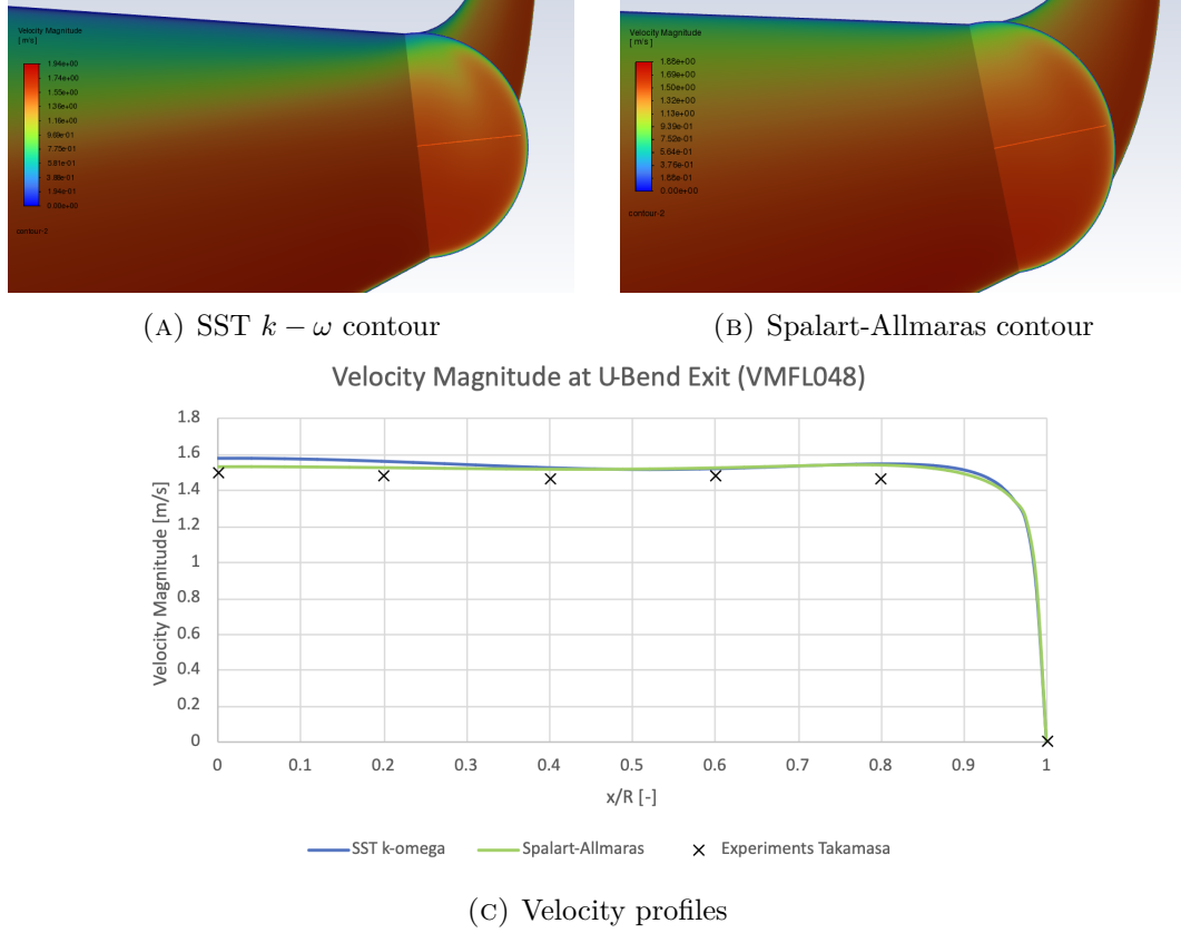
FIGURE 2.6: Flow predictions for a 180° U-bend ( R_c \approx 4.46D , Re_D \approx 44,700 , De \approx 15,000 ). The SA model matches the SST k - \omega contours and aligns with the experimental data from Takamasa and Kondo [53].
