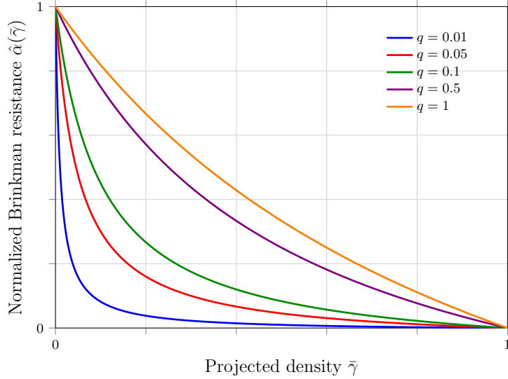
FIGURE 5.1: Normalized RAMP Brinkman resistance from Eq. 5.1 for q = \{0.01, 0.05, 0.1, 0.5, 1.0\} , adapted from Stolpe and Svanberg [50].
