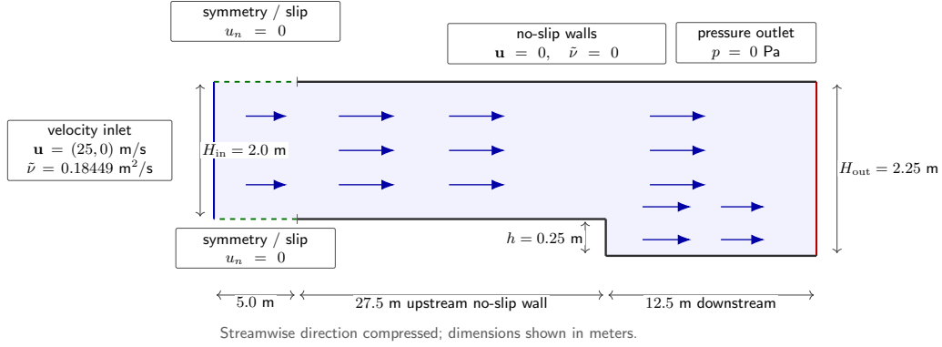
FIGURE 2.8: Backward-facing-step benchmark geometry and boundary conditions. The first 5.0 m of the upper and lower boundaries are treated as symmetry/slip segments, while all remaining solid boundaries are no-slip walls. The streamwise dimension is compressed for readability.
