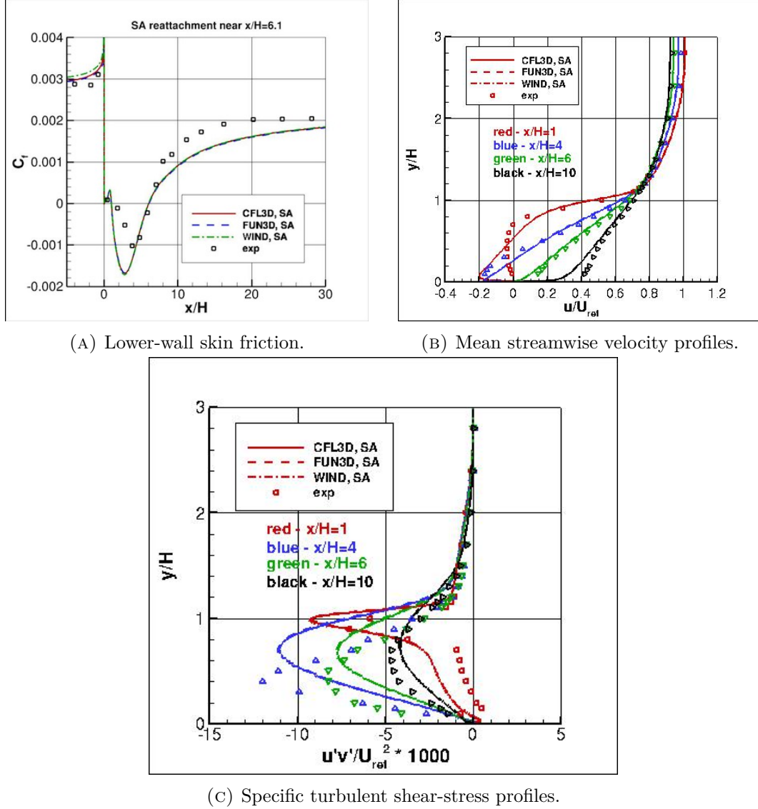
FIGURE 2.5: NASA Turbulence Modeling Resource comparison of SA predictions with the Driver-Seegmiller backward-facing-step experiment at Re_H \approx 36,000 [20, 36]. The skin-friction plot gives the reattachment behavior, while the velocity and turbulent shear-stress profiles show the quality of the separated-flow recovery.
