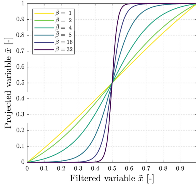
FIGURE 5.3: Heaviside projection from Eq. 5.23 at \eta = 0.5 for \beta = \{1, 2, 4, 8, 16, 32\} , reproduced from Ooms et al. [39].
