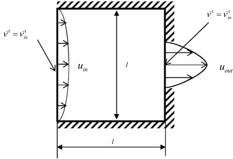
FIGURE 6.11: Geometry and boundary conditions for the diffuser benchmark from Yoon [60].
