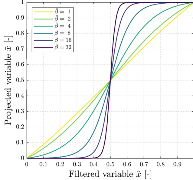
FIGURE 5.3: Heaviside projection from Eq. 5.18 at \eta = 0.5 for \beta = \{1, 2, 4, 8, 16, 32\} , reproduced from Ooms et al. [35].
