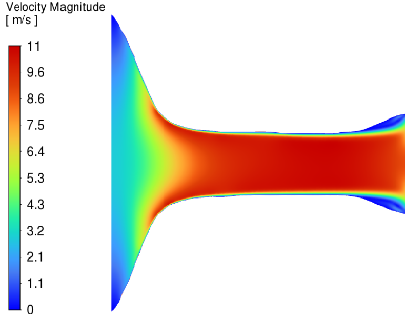
FIGURE E.7: Ansys-SA velocity-magnitude contour for the extracted velocity-outlet diffuser baseline. The low-speed region near the widened outlet motivates the pressure-outlet sensitivity study.
