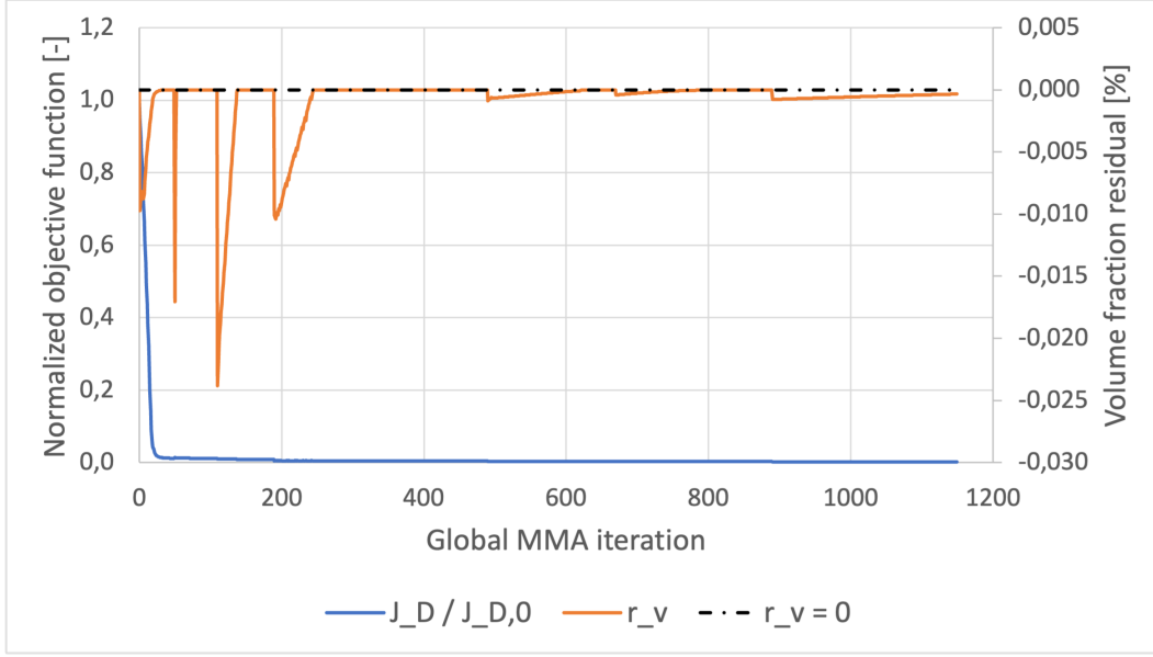
FIGURE E.8: Optimization convergence history for the turbulent pressure-outlet diffuser benchmark. The blue curve shows the normalized dissipation objective J_D/J_{D,0} , the orange curve shows the relative volume-fraction residual, and the dashed black line marks the active volume constraint.
