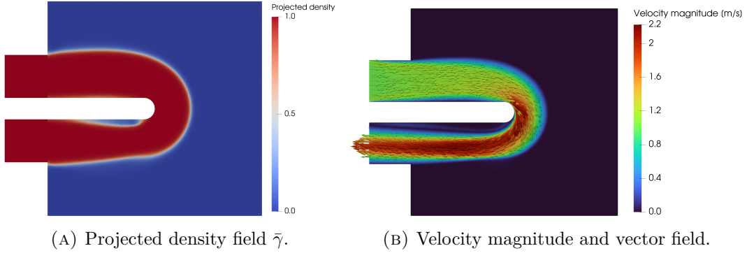
FIGURE 6.7: FEniCS-SA optimization result for the U-bend benchmark at V_f = 0.27 . Final objective value J_p = TBD Pa.
