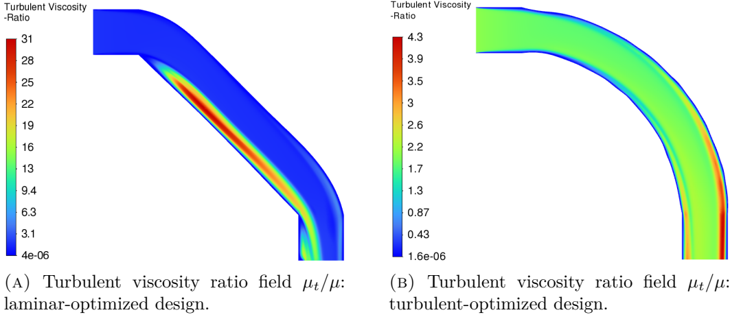
FIGURE 6.5: Turbulent viscosity ratio comparison for the pipe-bend designs, evaluated with an identical turbulent flow (SST k - \omega model).
