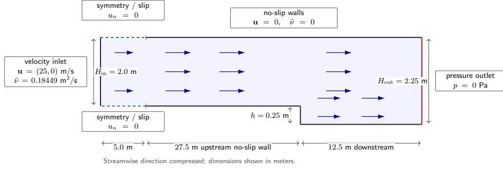
FIGURE A.1: Backward-facing-step benchmark geometry and boundary conditions, based on the configuration used by Marcibál and the associated code implementation [35, 30]. The first 5.0 m of the upper and lower boundaries are treated as symmetry/slip segments, while all remaining solid boundaries are no-slip walls. The streamwise dimension is compressed for readability.
