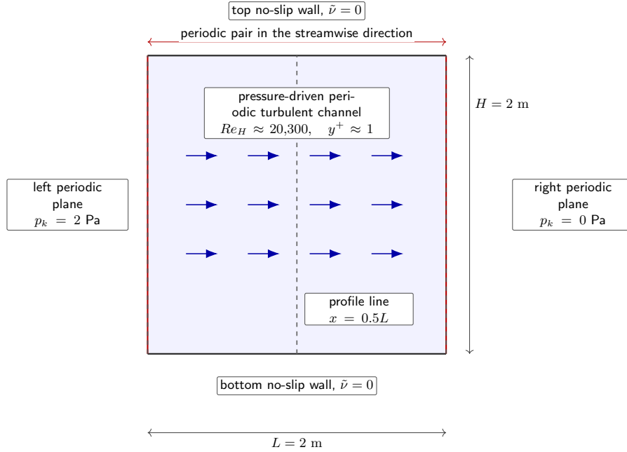
FIGURE 4.1: Pressure-driven periodic channel setup.
