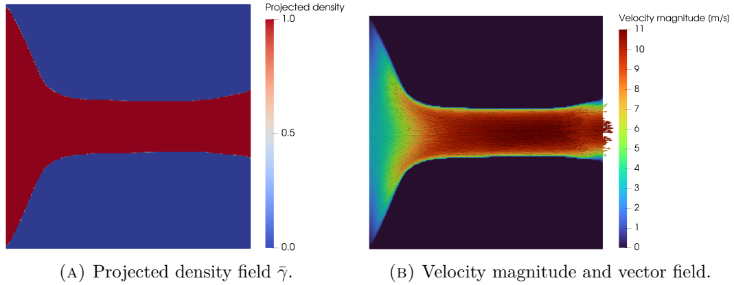
FIGURE 6.11: FEniCS-SA optimization result for the pressure-outlet diffuser at V_f = 0.30 . Final objective value J_D = 2.7664 \times 10^5 \text{ W/m} .
