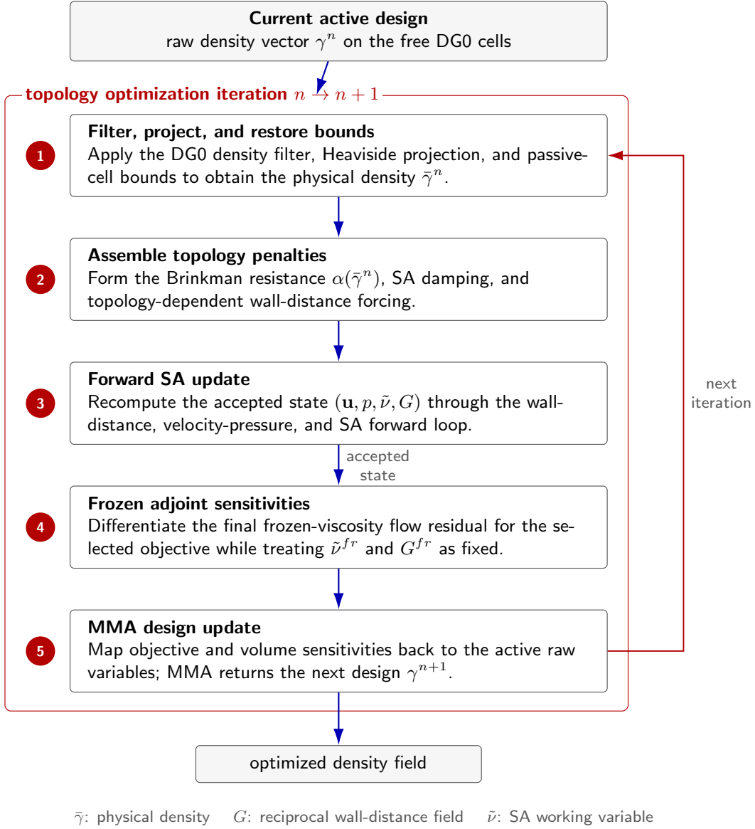
FIGURE 5.1: Algorithmic path of the density-based frozen-turbulence topology optimization loop.
