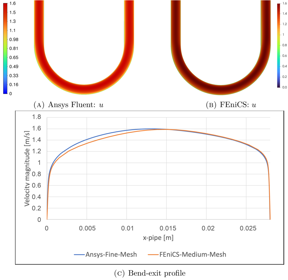
FIGURE 4.5: U-bend velocity validation.
