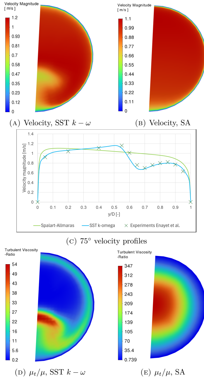
FIGURE 2.8: VMFL030 90° pipe-bend RANS comparison.
