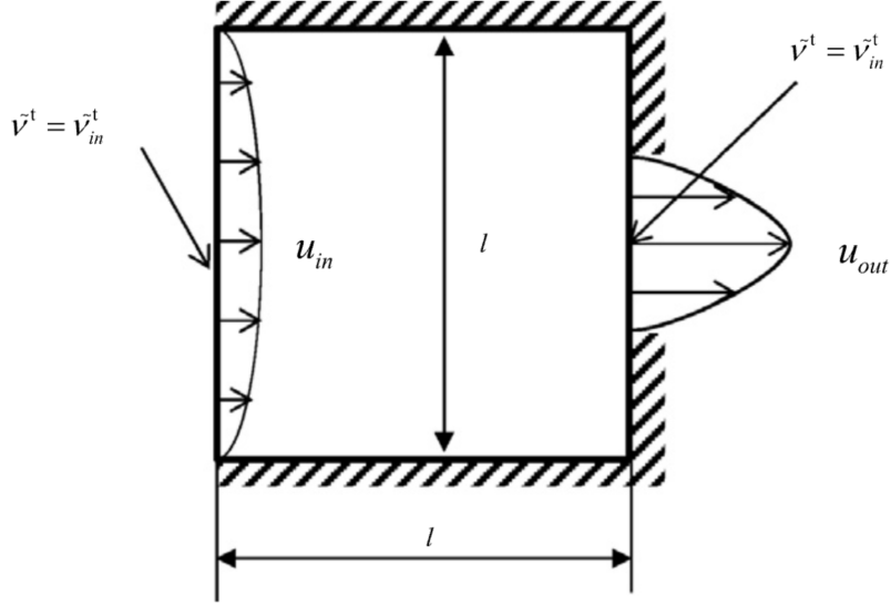
FIGURE E.5: Geometry and boundary conditions for the velocity-outlet diffuser baseline following Yoon [59]. Both inlet and outlet are prescribed by shifted parabolic velocity profiles.
