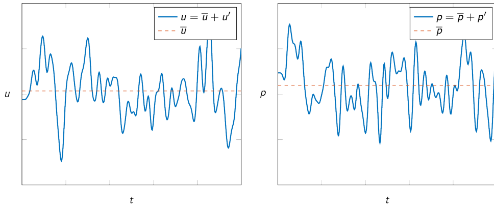
FIGURE 2.1: Reynolds decomposition of velocity and pressure signals. Adapted from [40].
