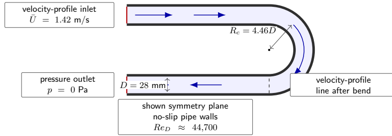
(A) VMFL048 3D U-bend.
