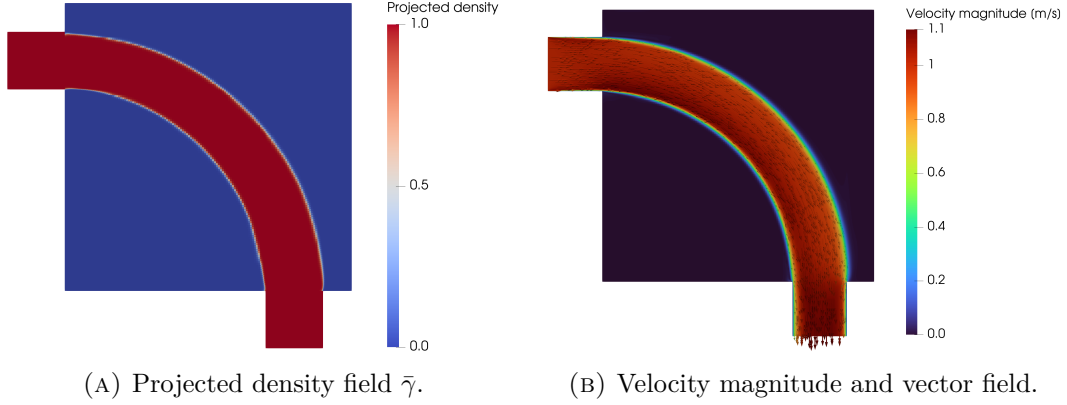
FIGURE 6.2: FEniCS-SA optimization result for the pipe-bend benchmark at V_f = 0.25 . Final objective value J_p = [TBD] Pa.
