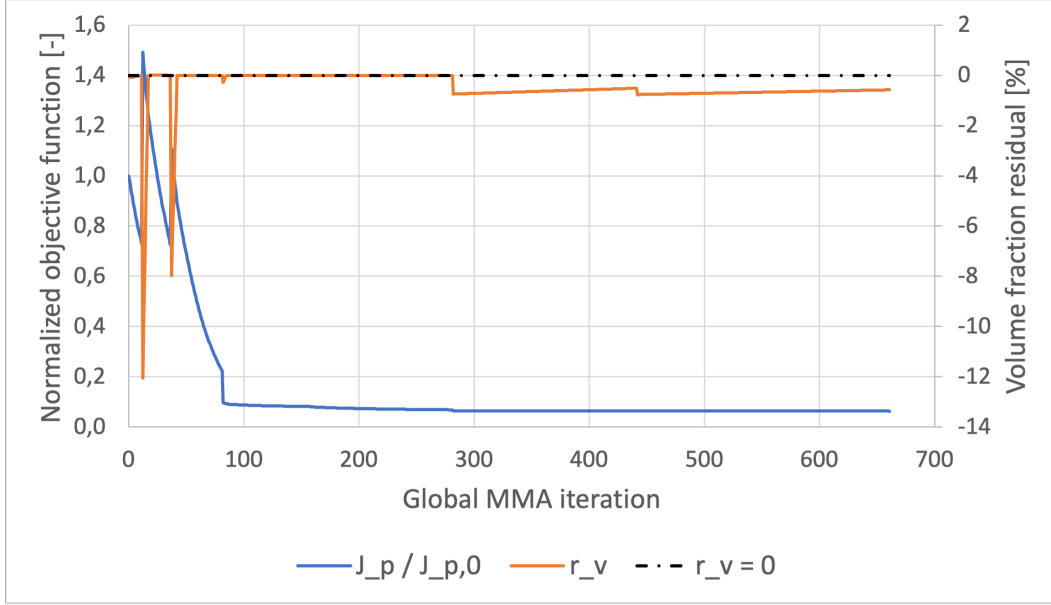
FIGURE E.4: FEniCS convergence history for the laminar U-bend topology-optimization run. The blue curve is the normalized inlet-pressure objective J_p/J_{p,0} , the orange curve is the relative volume-fraction residual, and the dashed black line marks the active volume constraint.
