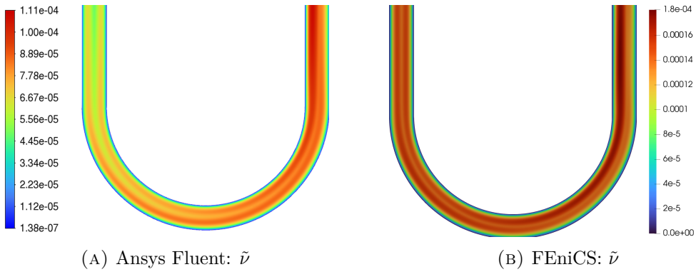
FIGURE 4.6: U-bend modified turbulent viscosity.
