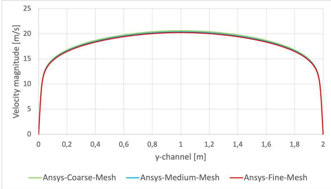
FIGURE C.2: Wall-normal velocity profiles extracted at x = 0.5L for the Coarse, Medium, and Fine grids in the Ansys periodic channel flow benchmark, demonstrating spatial convergence of the baseline data.
