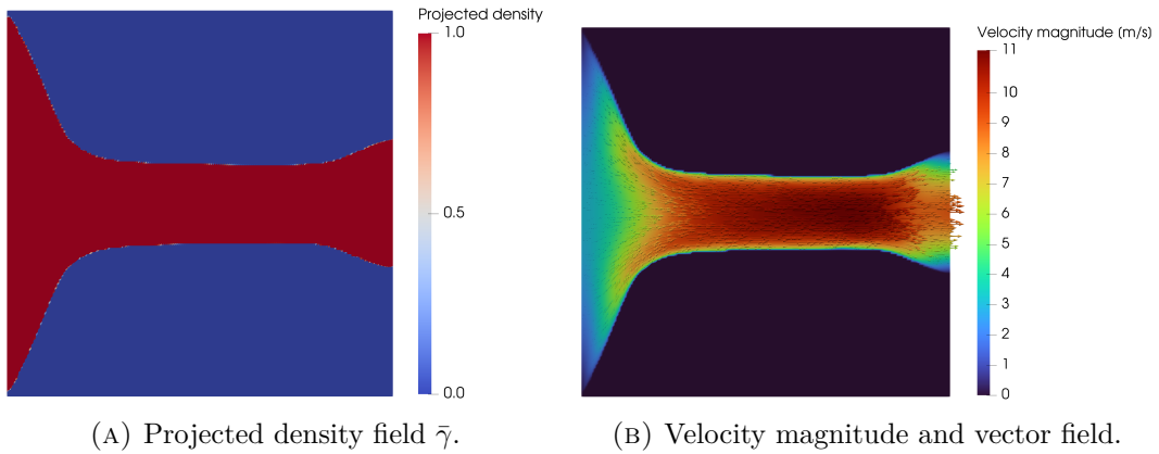
FIGURE E.6: FEniCS-SA result for the velocity-outlet diffuser baseline at V_f = 0.30 . Final objective value J_D = 3.1164 \times 10^5 W/m.
