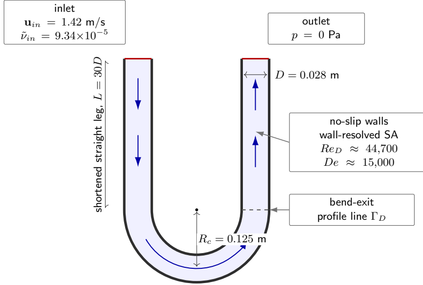
FIGURE 4.4: Shortened 2D U-bend verification setup.
