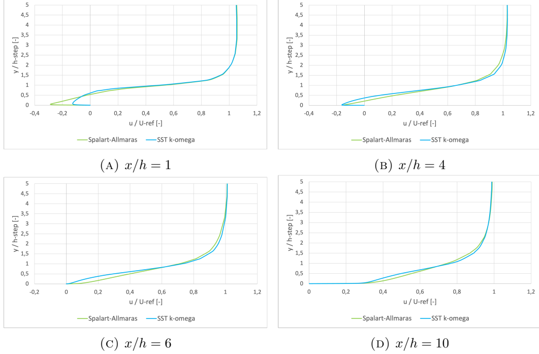
FIGURE A.4: Normalized streamwise velocity profiles for the backward-facing-step benchmark at four downstream stations. The comparison isolates model-form sensitivity by running SA and SST k - \omega on the same local backward-facing-step geometry and boundary conditions.
