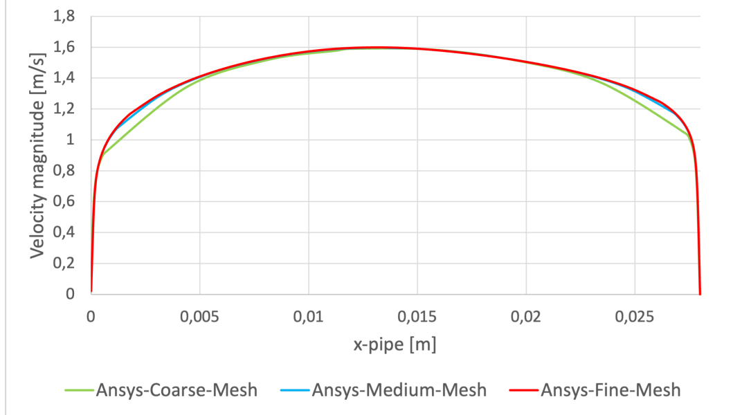
FIGURE C.4: Velocity profiles at the U-bend exit, extracted across the pipe diameter D = 0.028 m, for the Coarse, Medium, and Fine Ansys grids, demonstrating spatial convergence of the commercial baseline.
