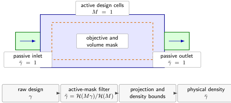
FIGURE D.2: Schematic active design region with passive inlet and outlet extensions. Passive cells are fixed by the density bounds but still participate in the forward flow solve.
