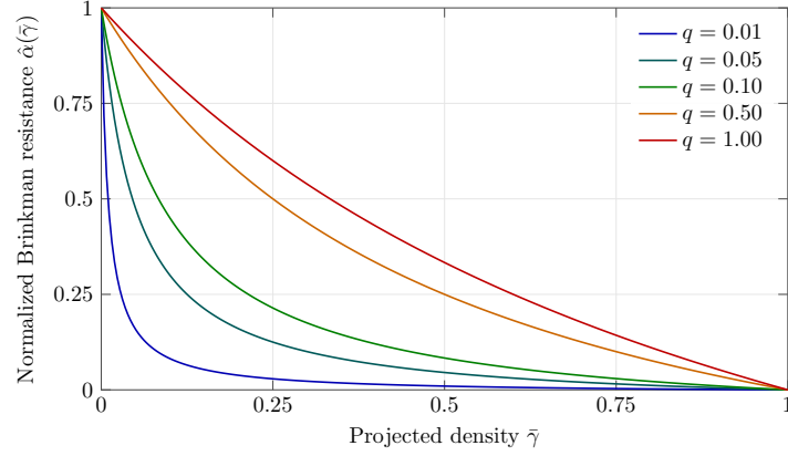
FIGURE D.1: Normalized RAMP Brinkman resistance from Eq. 5.1 for q = \{0.01, 0.05, 0.1, 0.5, 1.0\} .
