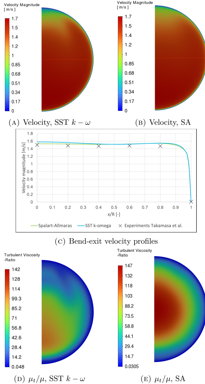
FIGURE 2.7: VMFL048 U-bend RANS comparison.
