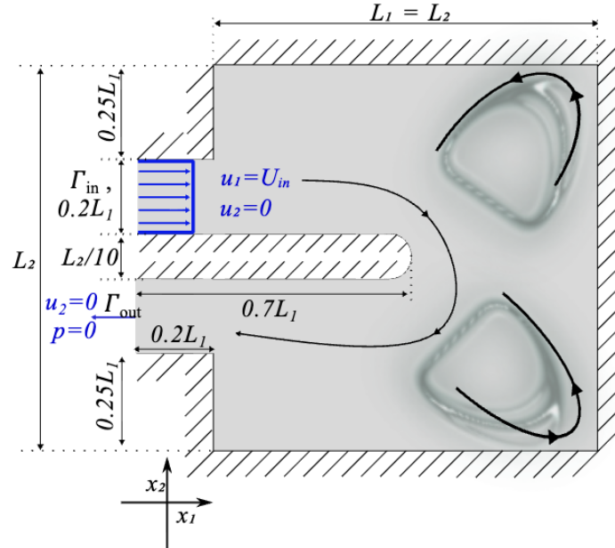
FIGURE 6.6: Geometry and boundary conditions for the U-bend benchmark from Bayat et al. [13].
