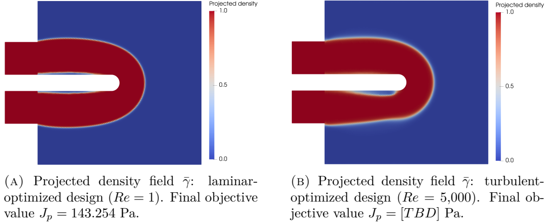
FIGURE 6.8: Laminar and turbulent topology comparison for the U-bend benchmark.
