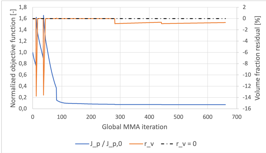
FIGURE E.2: FEniCS convergence history for the laminar pipe-bend topology-optimization run. The blue curve is the normalized inlet-pressure objective J_p/J_{p,0} , the orange curve is the relative volume-fraction residual, and the dashed black line marks the active volume constraint.
