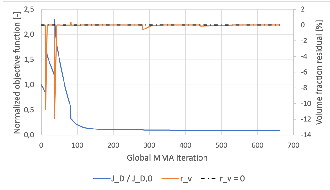
FIGURE E.9: FEniCS convergence history for the pressure-outlet laminar diffuser topology-optimization run. The blue curve is the normalized dissipation objective J_D/J_{D,0} , the orange curve is the relative volume-fraction residual, and the dashed black line marks the active volume constraint.
