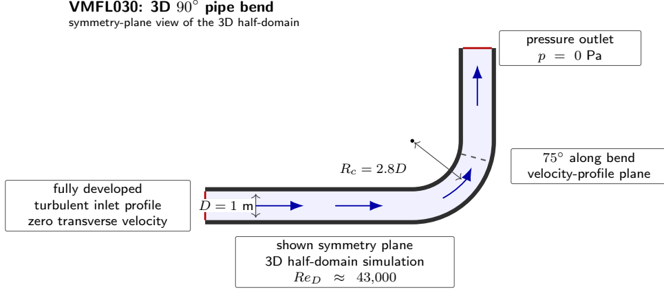
FIGURE 2.8: Geometry and boundary conditions for the VMFL030 3D 90° pipe-bend benchmark adopted from the Ansys Fluid Dynamics Verification Manual [8]. The schematic is not to scale.
