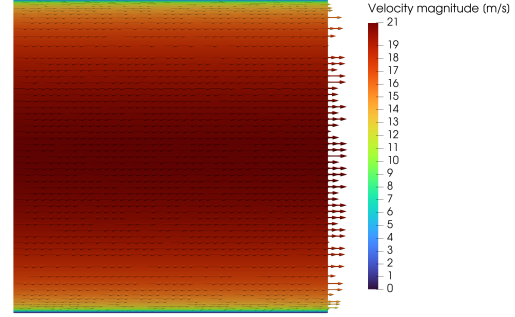
(B) FEniCS velocity magnitude contour
