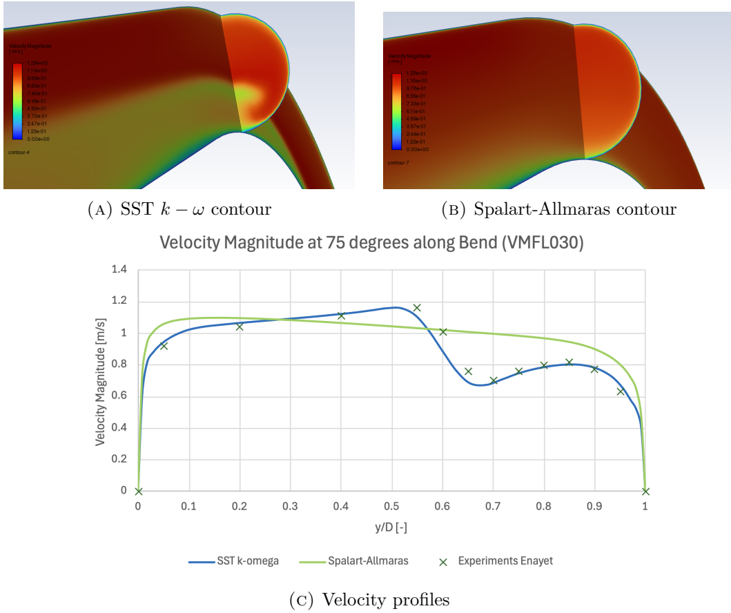
FIGURE 2.9: Flow predictions at the 75^\circ plane along the 90^\circ pipe bend ( R_c = 2.8D , Re_D \approx 43,000 , De \approx 18,000 ). The SA model over-smooths the velocity gradients near the inner wall, deviating from both the SST k - \omega model and the experimental data from Enayet et al. [22].
