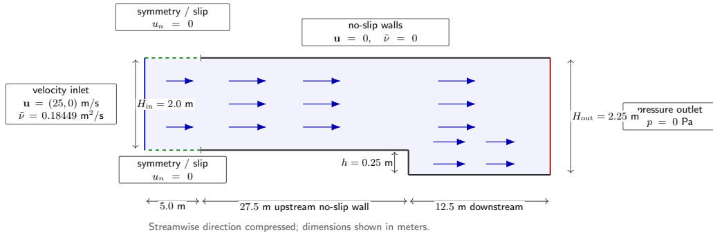
FIGURE 2.10: Backward-facing-step benchmark geometry and boundary conditions, based on the configuration used by Marcibál and the associated GitHub implementation [35, 30]. The first 5.0 m of the upper and lower boundaries are treated as symmetry/slip segments, while all remaining solid boundaries are no-slip walls. The streamwise dimension is compressed for readability.
