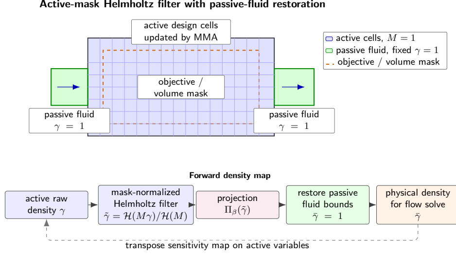
FIGURE 5.2: Schematic of active design cells, passive fluid cells, objective and volume masks, and the active-mask-normalized Helmholtz filtering chain. The filter concept follows the PDE-filter formulation of Lazarov and Sigmund and the regularization motivation of Bourdin [33, 15].
