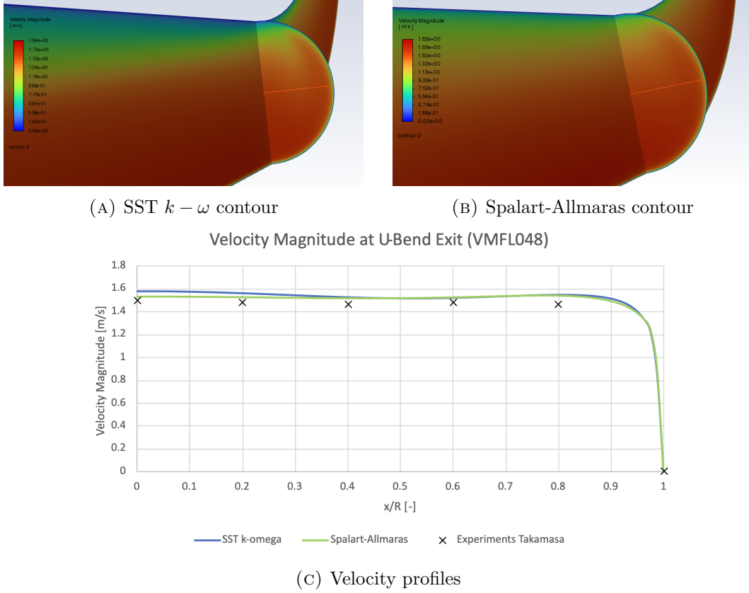
FIGURE 2.7: Flow predictions for a 180^\circ U-bend ( R_c \approx 4.46D , Re_D \approx 44,700 , De \approx 15,000 ). The SA model matches the SST k - \omega contours and aligns with the experimental data from Takamasa and Kondo [55].
