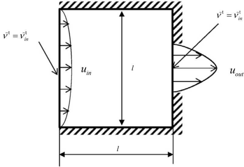
FIGURE 6.11: Geometry and boundary conditions for the diffuser benchmark from Yoon [57].
