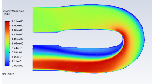
(A) Velocity magnitude field u : laminar-optimized design.
