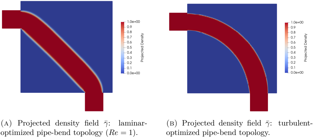
FIGURE 6.4: Laminar and turbulent topology comparison for the pipe-bend benchmark.
