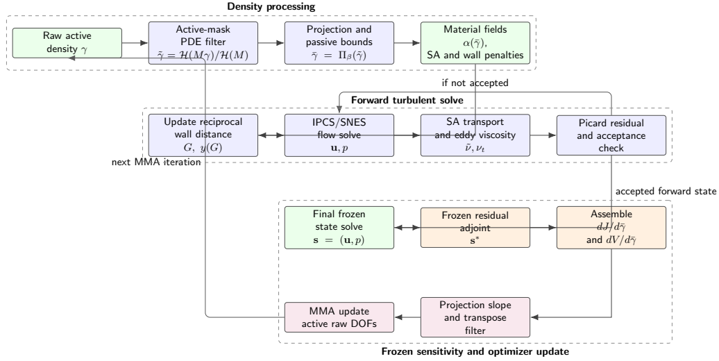
FIGURE 4.4: Workflow of the density-based frozen-turbulence topology optimization algorithm. The forward turbulence fields are updated in the flow loop, while the adjoint differentiates only the final frozen-viscosity residual.
