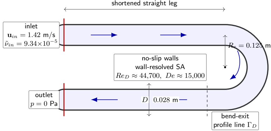
FIGURE 5.3: Schematic of the shortened 2D U-bend verification setup based on the VMFL048 operating point from the Ansys verification manual [8]. The profile line \Gamma_D is used for the bend-exit velocity comparison.
