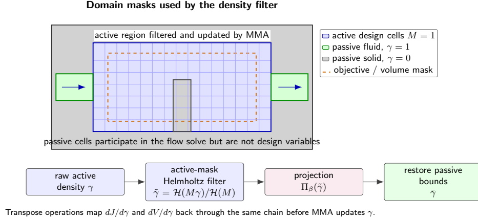
FIGURE 4.2: Schematic of active design cells, passive fluid/solid cells, objective and volume masks, and the active-mask-normalized Helmholtz filtering chain. The filter concept follows the PDE-filter formulation of Lazarov and Sigmund and the regularization motivation of Bourdin [30, 15].
