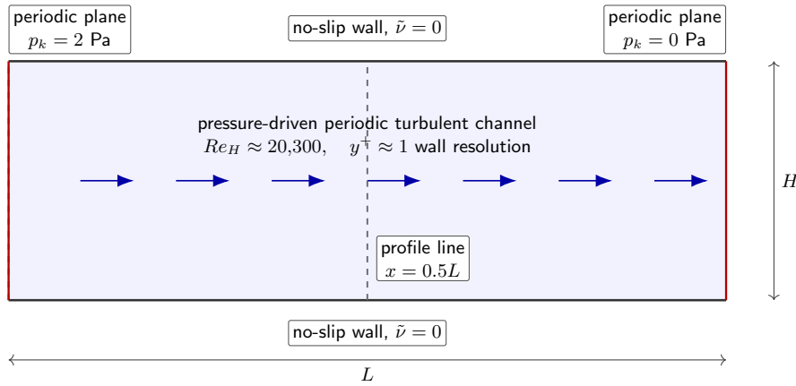
FIGURE 5.1: Schematic of the pressure-driven periodic channel verification setup. The vertical dashed line marks the mid-plane profile extraction location used for the FEniCS–Ansys comparison.
