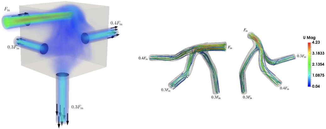
FIGURE 1.2: Topology optimized manifolds with turbulent flow. Adapted from Dilgen et al. [16].
