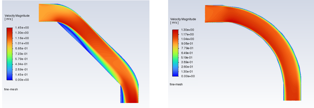
(A) Velocity magnitude field u : laminar-optimized design.
