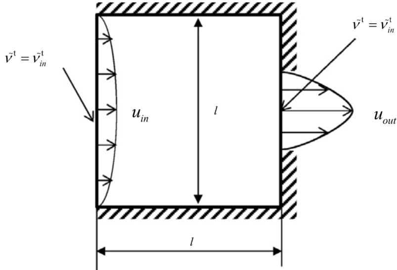
FIGURE 6.11: Geometry and boundary conditions for the diffuser benchmark from Yoon [47].
